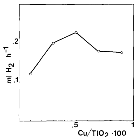
Fig. 5. Rate of hydrogen photoproduction from water-methanol vs. the Cu:TiO 2 ratio (amount of TiO 2 =0.005 g)
