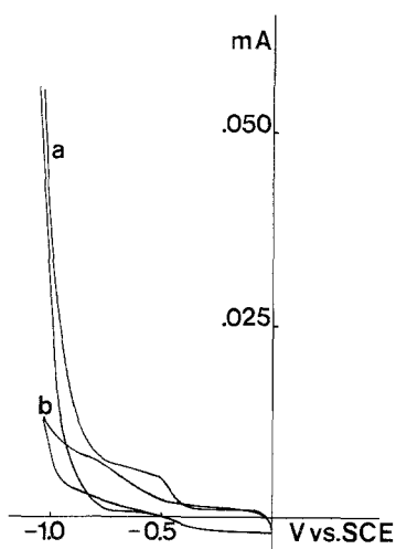
Fig. 3. I - V curve for a graphite electrode immersed in \text{Cu}/\text{TiO}_2 suspension in water-methanol(3:1)-0.5m KCl (curve a ), and the electrode immersed in a \text{TiO}_2 suspension in water-methanol-KCl (curve b )
