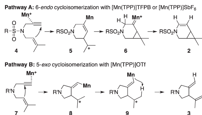
Scheme 2. Plausible Reaction Pathways
