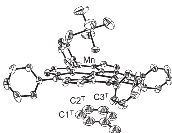
Figure 1. ORTEP drawing of [Mn(TPP)]SbF 6 (toluene).
