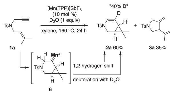
Scheme 4. Cycloisomerization of 1a in the Presence of D 2 O
