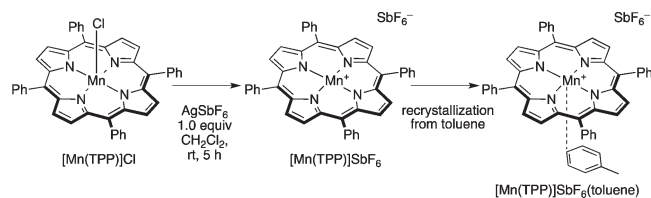
Scheme 1. Synthesis of [Mn(TPP)]SbF 6 Catalyst
