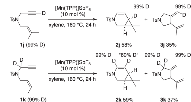
Scheme 3. Reaction of Deuterium-Labeled Enynes
