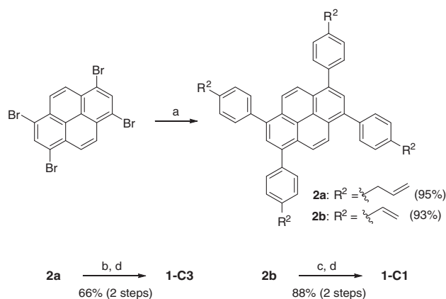
Scheme 1. Synthetic routes to newly designed TPPy-bridged alkoxy silane precursors; 1-C3 and 1-C1 . Reagents and conditions: (a) [\text{Pd}(\text{PPh}_3)_4] , \text{K}_2\text{CO}_3 (aq), 4-allylphenylboronic acid, 1,4-dioxane, 90^\circ\text{C} for 2a , [\text{Pd}(\text{PPh}_3)_4] , \text{K}_3\text{PO}_4 (aq), 4-vinylphenylboronic acid, 1,4-dioxane, 80^\circ\text{C} for 2b ; (b) \text{H}_2[\text{PtCl}_6] \cdot 6\text{H}_2\text{O} , \text{HSiCl}_3 , benzene, 40^\circ\text{C} ; (c) [\text{PdCl}(\pi\text{-C}_3\text{H}_5)_2] , rac -H-MOP, \text{HSiCl}_3 , benzene, 40^\circ\text{C} ; (d) i -PrOH, pyridine, \text{CH}_2\text{Cl}_2 , 0^\circ\text{C} –rt.
