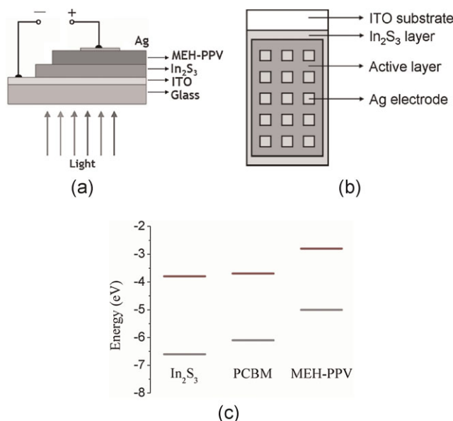
Figure 1 (online colour at: www.pss-a.com ) (a) Device structure, (b) schematic of the top of the device and (c) HOMO-LUMO energy levels of MEH-PPV and PCBM, and the position of conduction band minimum and valence band maximum of \text{In}_2\text{S}_3 .
