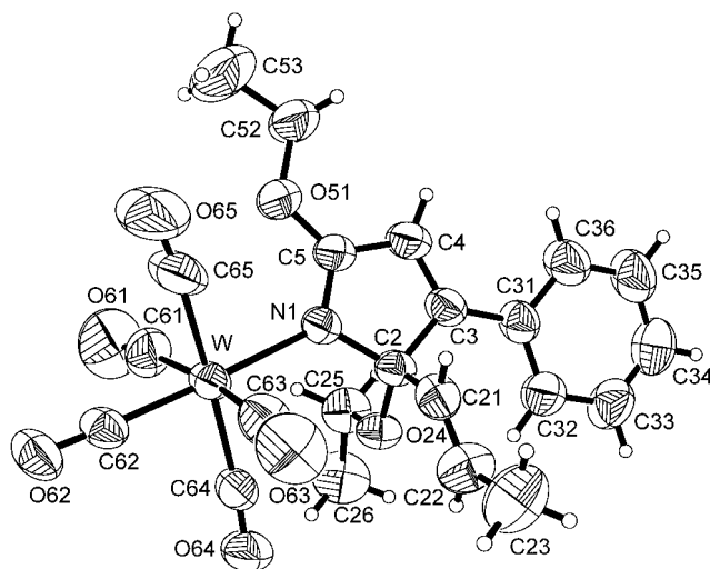
Figure 1. Molecular structure of the 5-aza-1-tungsta-1,3,5,7-tetraene 9b .
