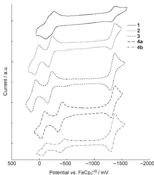
Figure 3. Cyclic voltammograms of 1 , 2 , 3 , 4a and 4b ( \text{CH}_2\text{Cl}_2 , 0.1 M [\text{nBu}_4\text{N}]^+[\text{PF}_6]^- , 50 \text{mVs}^{-1} ) with \text{Cp}_2\text{Co}^{+/0} as an internal reference ( -1320 \text{ mV} versus \text{FeCp}_2^{+/0} ).
