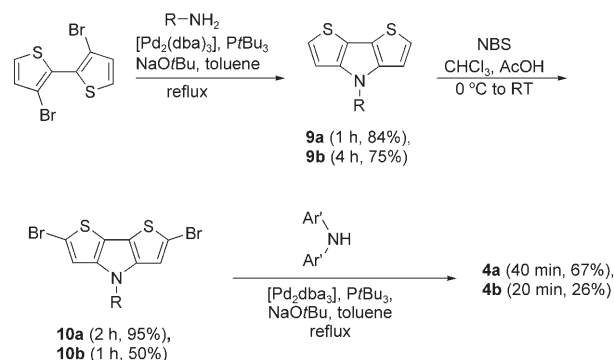
Scheme 2. Synthesis of bis(diarylamino)dithienopyrroles 4a and 4b (Ar' = MeOC 6 H 4 ; R = 4- n BuC 6 H 4 for 4a , 9a and 10a ; R = 4- t Bu for 4b , 9b and 10b ).
