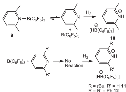
Scheme 4. Reactions of Substituted-Pyridines with H_2
