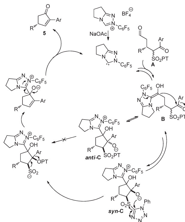
Scheme 4. Proposed Mechanism for the NHC-Catalyzed Benzoin Condensation and Subsequent Smiles Rearrangement
