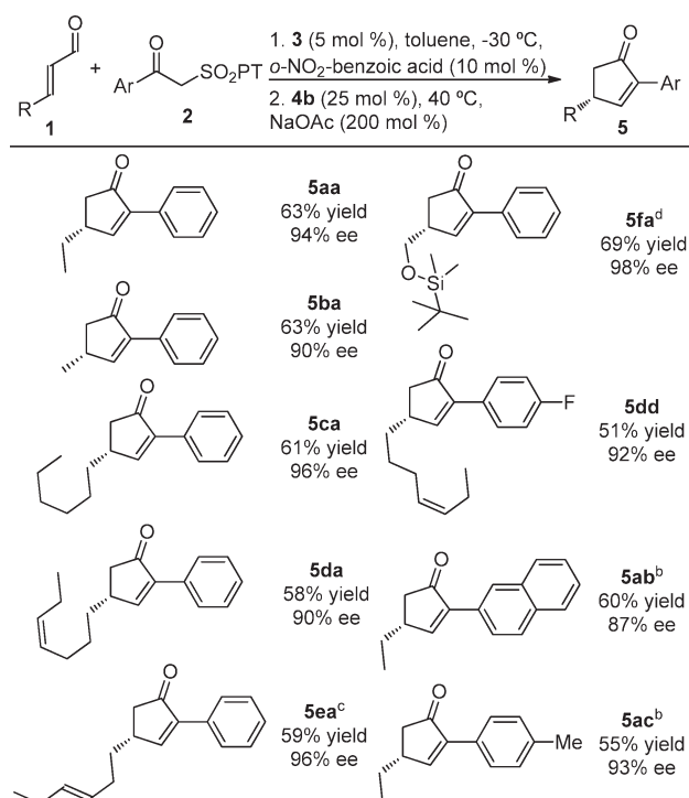
Scheme 2. Scope of the Organocatalytic Formation of 2,4-Disubstituted Cyclopent-2-enones 5 a
