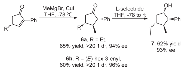
Scheme 3. Transformation of the Obtained Products 5 a
