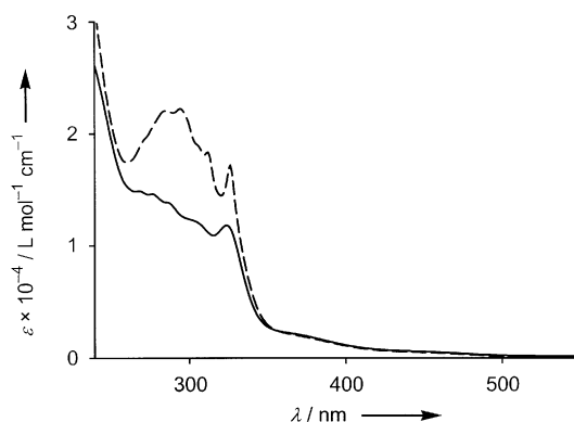
Figure 5. Absorption spectra of the semi-dumbbell compounds 18 (---) and 24 (—) recorded in MeCN at room temperature.
