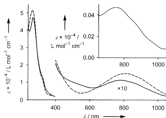
Figure 7. Absorption spectra of the [2]pseudorotaxanes 18 ⊂ CBPQT 4+ (—) and 24 ⊂ CBPQT 4+ (---) recorded in MeCN at room temperature. The contribution of the CT band of the “alongside” interacting MPTTF unit in 18 ⊂ CBPQT · RED 4+ is shown in the inset. For more details, see text.
