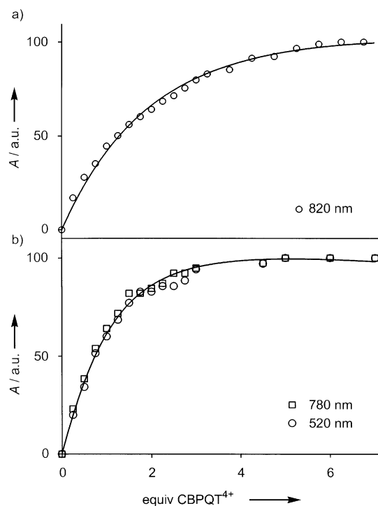
Figure 6. Titration curves for the formation of the [2]pseudorotaxanes a) 24 ⊂ CBPQT 4+ and b) 18 ⊂ CBPQT 4+ in MeCN at room temperature. For more details, see text.
