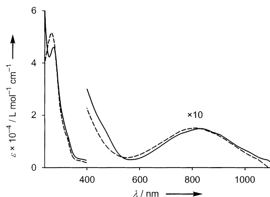
Figure 9. Comparison of the absorption spectra of the single-station [2]rotaxane 1^{4+} (—) and the [2]pseudorotaxane 24 \subset \text{CBPQT}^{4+} (---) recorded in MeCN at room temperature.
