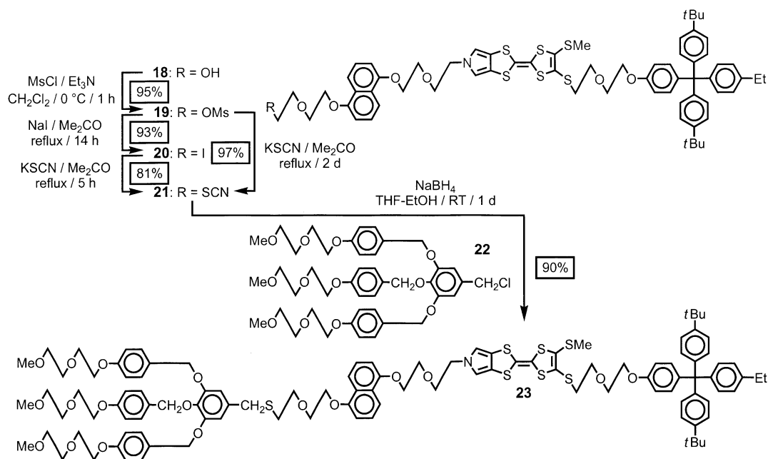
Scheme 5. Synthesis of the dumbbell compound 23 .
