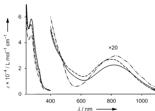
Figure 10. Comparison of the absorption spectra of the single-station [2]rotaxane 1^{4+} (- · -) and the two-station [2]rotaxanes 2^{4+} (—) and 3^{4+} (---) recorded in MeCN at room temperature.
