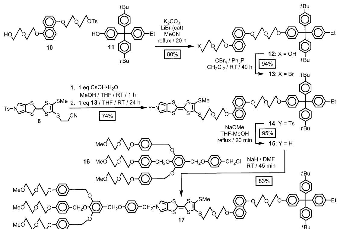
Scheme 3. Synthesis of the dumbbell compound 17 .
