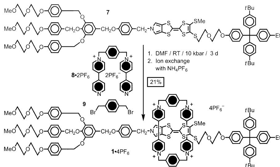
Scheme 2. Synthesis of the single-station [2]rotaxane 1 \cdot 4\text{PF}_6 .
