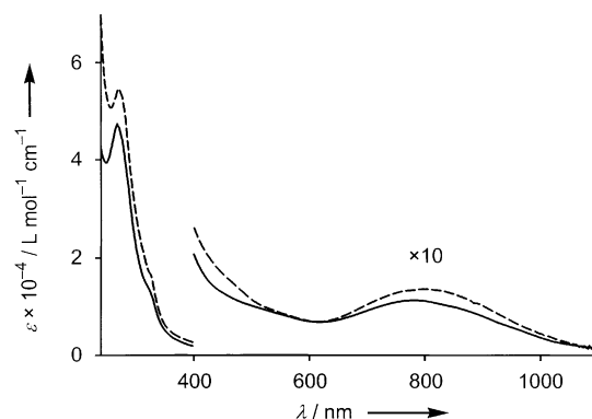
Figure 11. Comparison of the absorption spectra of the two-station [2]rotaxane 3^{4+} (---) and the [2]pseudorotaxane 18 \subset \text{CBPQT}^{4+} (—) recorded in MeCN at room temperature.
