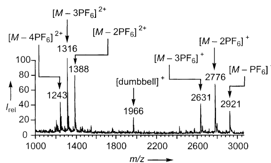
Figure 2. FAB-MS spectrum of the [2]rotaxane 2 ·4PF 6 .
