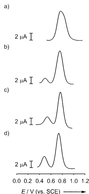
Figure 15. DPV peaks in MeCN solutions of a) the single-station [2]rotaxane \mathbf{1}^{4+} , b) the two-station [2]rotaxane \mathbf{2}^{4+} , c) the two-station [2]rotaxane \mathbf{3}^{4+} , and d) the [2]pseudorotaxane \mathbf{18} \subset \text{CBPQT}^{4+} . The current intensity has been corrected to take into account differences in diffusion coefficients and concentrations.
