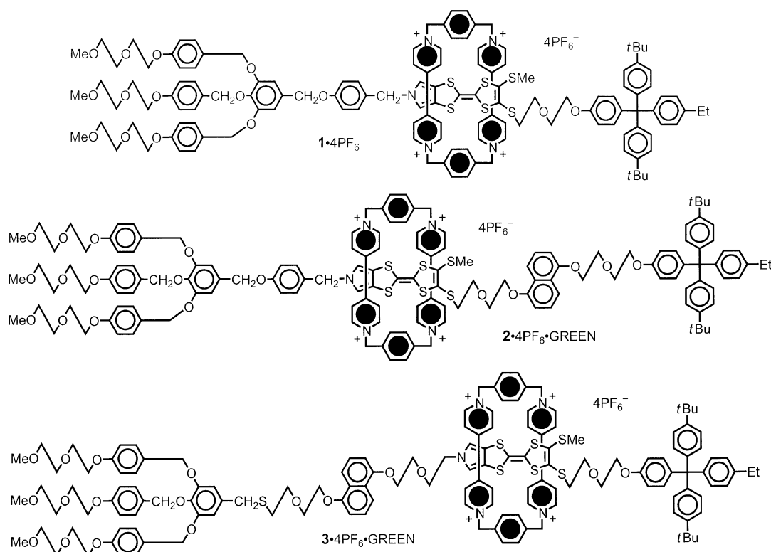
Figure 1. Molecular formulas of the single-station [2]rotaxane 1 ·4PF 6 , the slow two-station [2]rotaxane 2 ·4PF 6 , and the fast two-station [2]rotaxane 3 ·4PF 6 (only one translational isomer is shown in each case).
