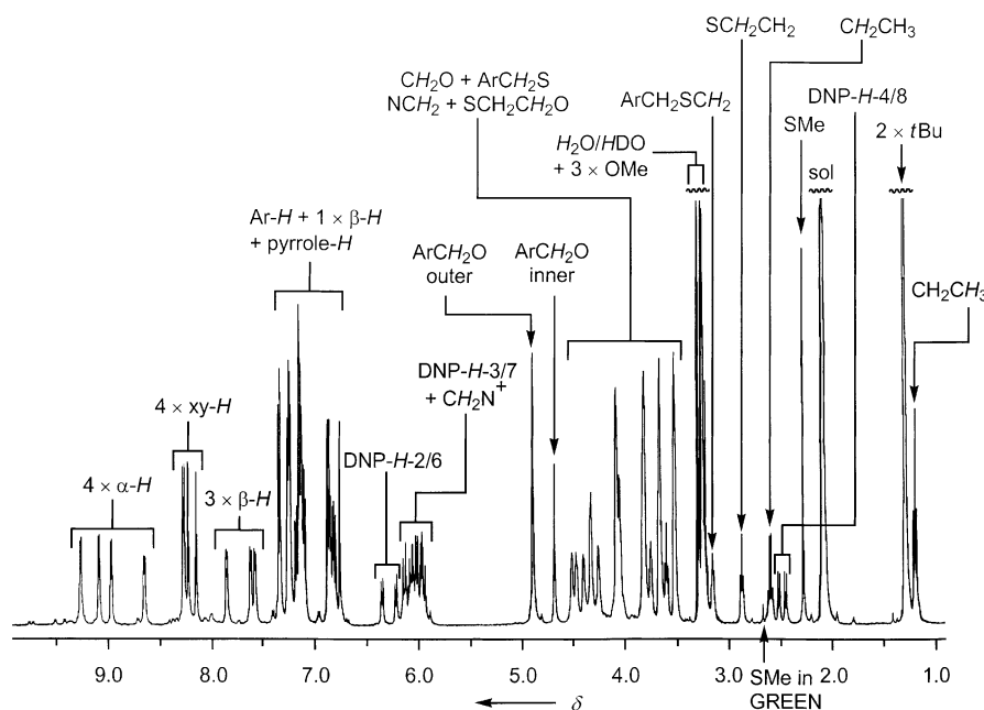
Figure 19. Full ^1\text{H} NMR spectrum (500 MHz) of the fast two-station [2]rotaxane 3 ^{4+} recorded in \text{CD}_3\text{COCD}_3 at 245 K.
