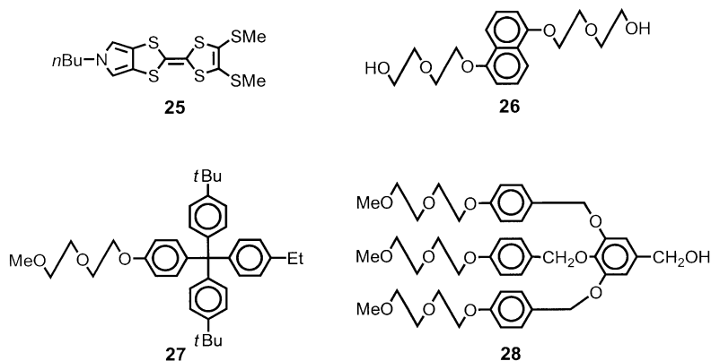
Figure 3. Molecular formulas of the model compounds of the \pi -electron donor stations ( 25 and 26 ) and the stoppers ( 27 and 28 ) of the dumbbell-shaped components of the [2]rotaxanes shown in Figure 1.
