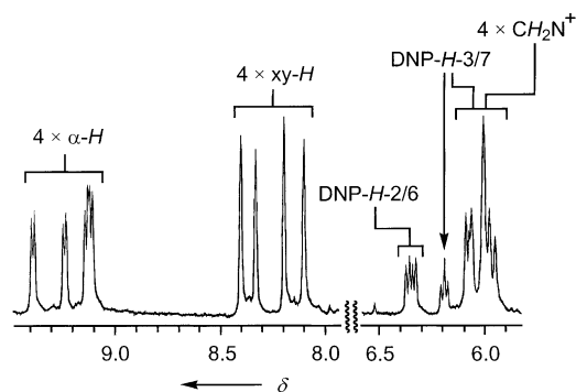
Figure 22. Partial ^1\text{H} NMR spectrum of the isolated [2]rotaxane 2 \cdot \text{RED}^{4+} recorded at 500 MHz in \text{CD}_3\text{COCD}_3 at 225 K.
