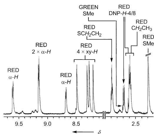
Figure 17. Partial ^1\text{H} NMR spectrum (500 MHz) of the 1:1 complexes formed between the semi-dumbbell compound 18 and \text{CBPQT}^{4+} recorded in \text{CD}_3\text{COCD}_3 at 245 K.
