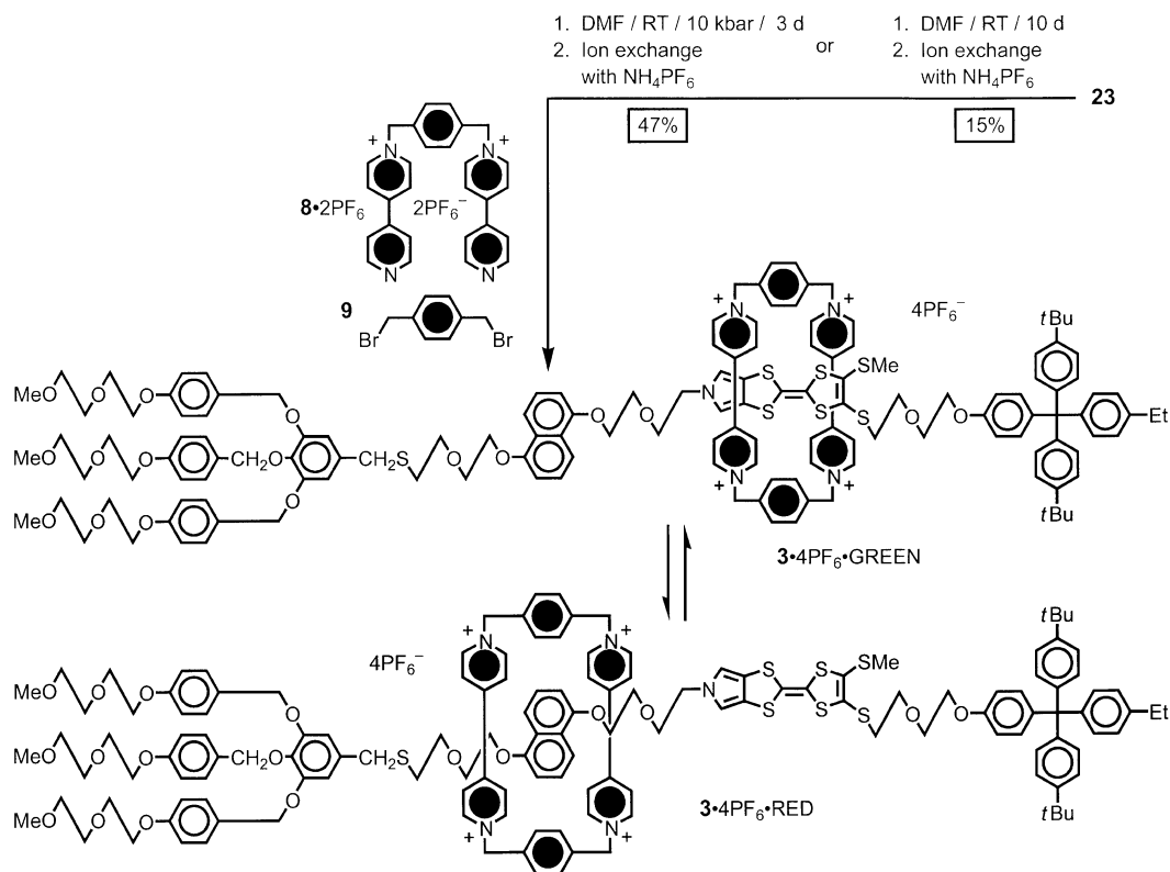
Scheme 6. Synthesis of the fast two-station [2]rotaxane 3 ·4PF 6 − .
