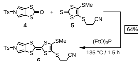
Scheme 1. Synthesis of the asymmetric MPTTF building block 6 .
