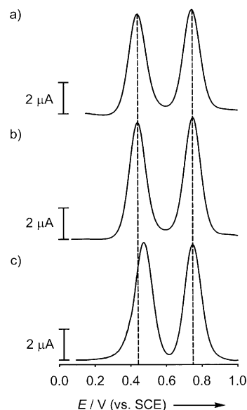
Figure 13. DPV peaks in MeCN solutions of a) the MPTTF model compound 25 , b) the semi-dumbbell compound 24 , and c) the [2]pseudorotaxane 24 ⊂ CBPQT 4+ . The current intensity has been corrected to take into account differences in diffusion coefficients and concentrations.
