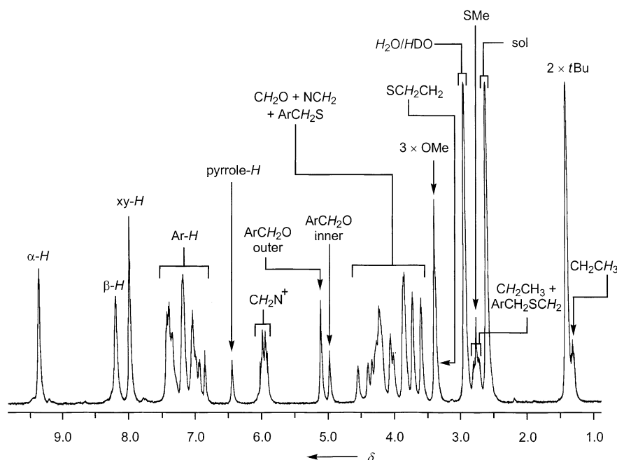
Figure 20. Full 1 H NMR spectrum (500 MHz) of the fast two-station [2]rotaxane 3 4+ recorded in CD 3 SOCD 3 at 400 K.
