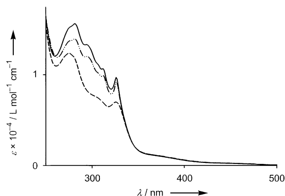
Figure 8. Absorption spectra of the dumbbell compounds 7 (---), 17 (—), and 23 (- · -) recorded in MeCN at room temperature.
