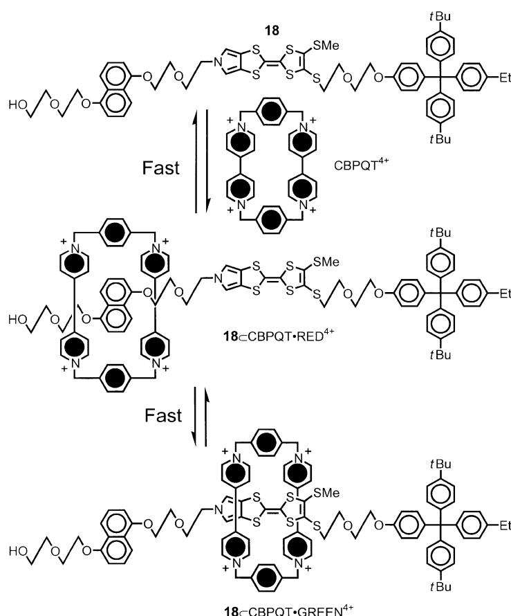
Scheme 8. Self-assembly of the two-station [2]pseudorotaxane 18 \subset \text{CBPQT}^{4+} .
