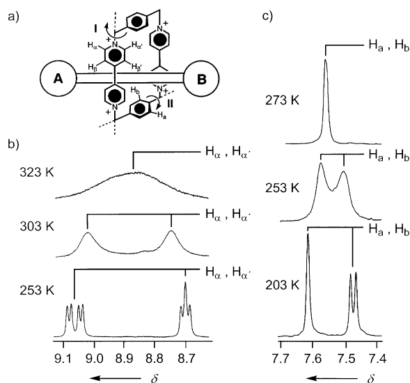
Figure 21. a) A schematic representation of the pyridinium unit rotation process (I) occurring in the bipyridinium units present in the tetracationic cyclophane component of the single-station [2]rotaxane 1^{4+} and the p -xylyl unit rotation process (II) occurring in the tetracationic cyclophane component of 1^{4+} . Rotation of the pyridinium units around the axis of the bipyridinium units brings about the exchange of H_{\alpha} with H_{\alpha'} and H_{\beta} with H_{\beta'} . Rotation of the p -xylyl units around their substituted axis causes exchange between H_a and H_b . Partial variable temperature ^1\text{H} NMR spectra (500 MHz) of a \text{CD}_3\text{COCD}_3 solution of the single-station [2]rotaxane 1^{4+} of b) the \alpha -bipyridinium region and c) the p -xylyl region.
