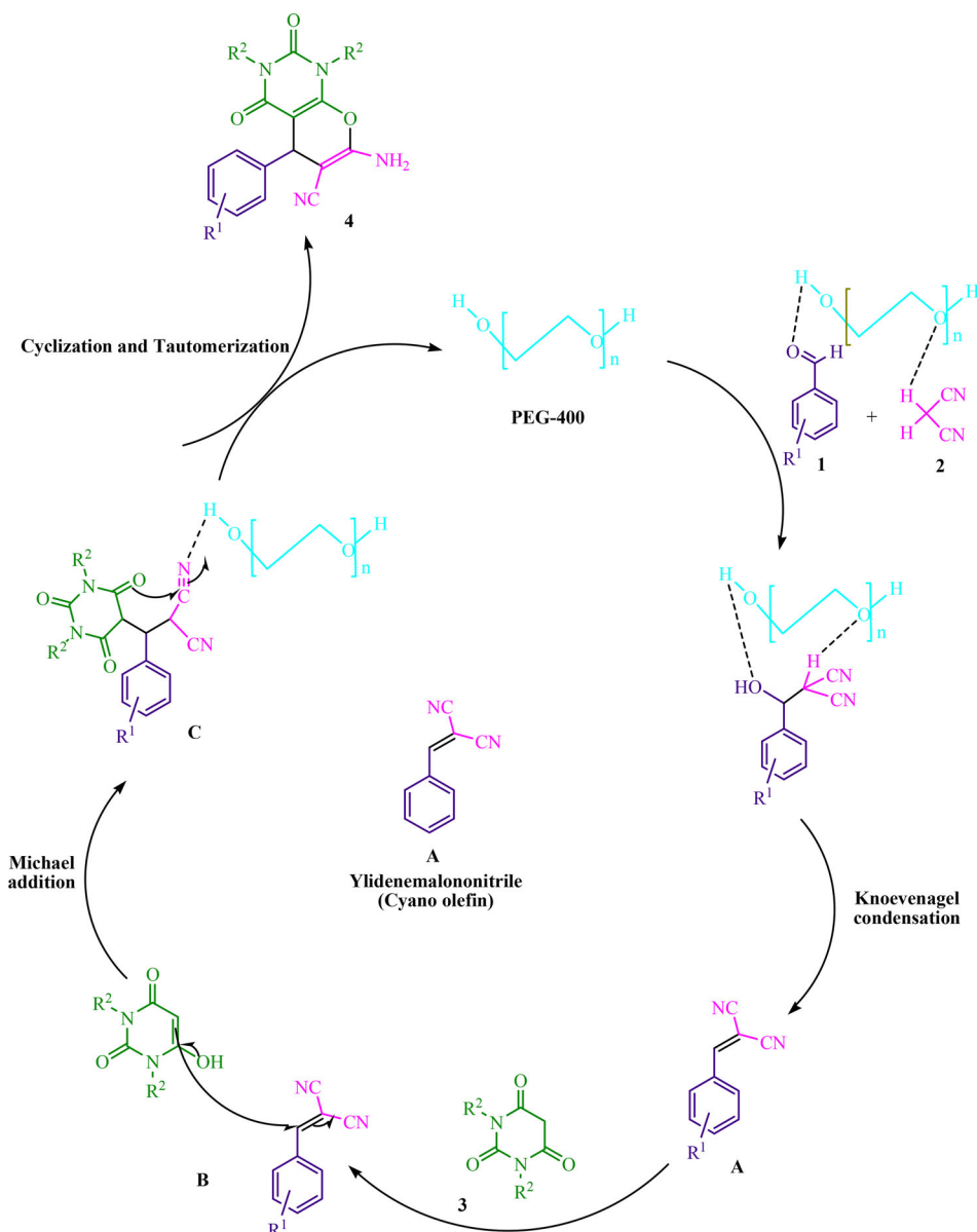
Scheme 2. Proposed mechanistic route for the synthesis of pyrano[2,3-d]pyrimidine scaffolds.
