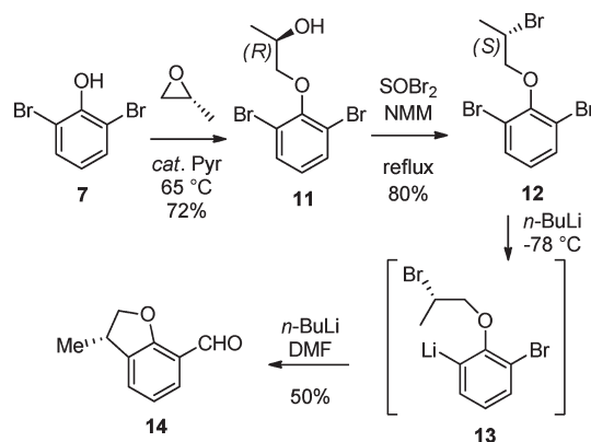
Scheme 3. Synthesis of ( S )-3-Methyldihydrobenzofuran-7-carboxaldehyde 14
