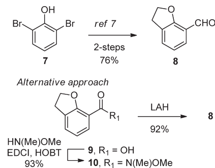
Scheme 2. Synthesis of Dihydrobenzofuran-7-carboxaldehyde 8
