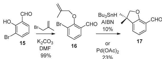
Scheme 4. Initial Attempts for the Synthesis of 3,3-Dimethyldihydrobenzofuran-7-carboxaldehyde 17
