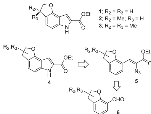
Scheme 1. New 4,5-Fused Dihydrofurano Indole Systems and Proposed Retrosynthetic Analysis for Their Synthesis
