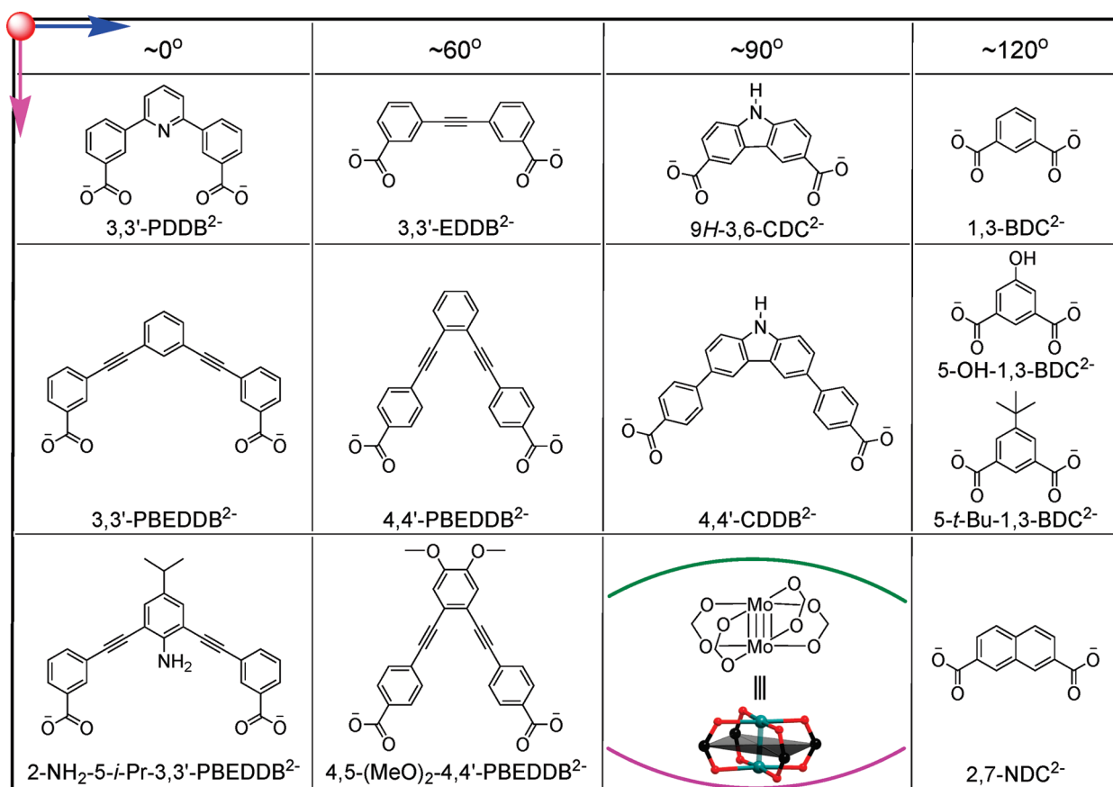
Figure 2. \text{Mo}_2(\text{O}_2\text{C}-)_4 cluster and bridging dicarboxylate ligands with different bridging angles, sizes, and nonbridging functional groups used in this work.
