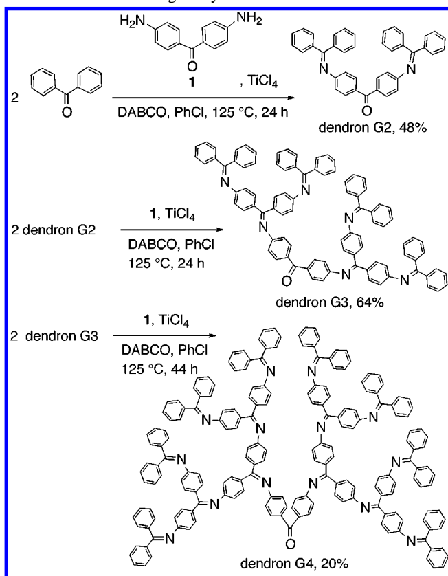
Scheme 1 Convergent Synthesis of the DPA Dendrons
