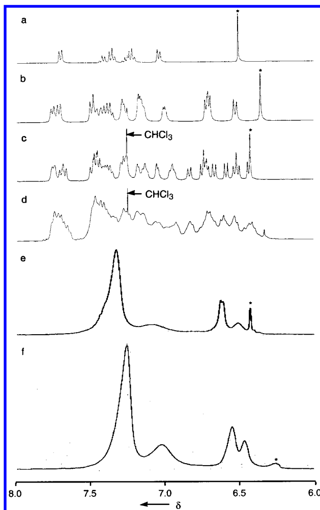
Figure 2. The ^1\text{H} NMR spectra of DPAs (a) G1, (b) G2, (c) G3, and (d) G4 in \text{CDCl}_3 at 30 ^\circ\text{C} and those of DPAs (e) G3 and (f) G4 in \text{DMSO}-d_6 at 130 ^\circ\text{C} . The marked peaks (*) are attributed to the four protons of the phenyl ring in the core of the DPAs.
