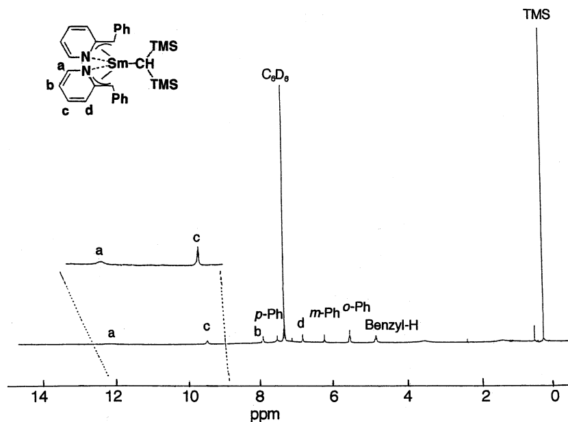
Fig. 2. ^1\text{H-NMR} spectrum of (2\text{-pyridylbenzyl})_2\text{SmCH}(\text{SiMe}_3)_2 3.
