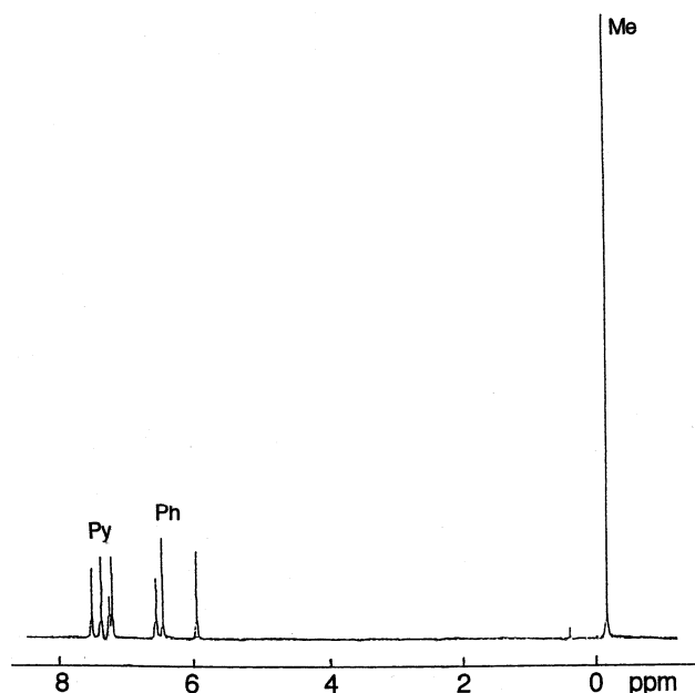
Fig. 5. ^1\text{H} -NMR spectrum of [(2\text{-pyr})_2\text{CPh}]_2\text{Yb}(\mu\text{-Me})_2\text{AlMe}_2 5 .
