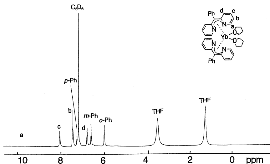
Fig. 3. ^1\text{H} -NMR spectrum of [(2\text{-Pyr})_2\text{CPh}]_2\text{Yb}(\text{THF})_2 4.
