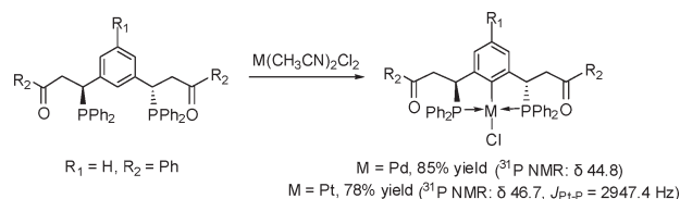
Scheme 3. Synthesis of Chiral PCP Pincer Complexes
