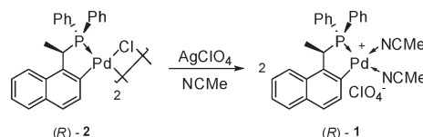
Scheme 1. Formation of the Phosphapalladacycle Catalyst ( R )- 1
