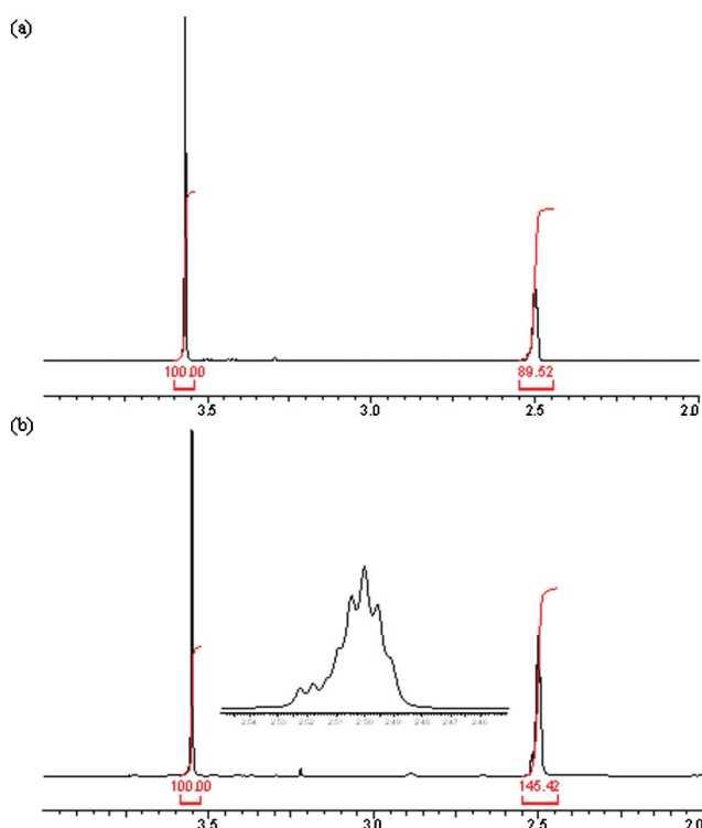
Fig. 1 (a) 1 H NMR spectrum of a mixture of [D 6 ]DMSO (550 μL, 7.775 mmol, δ = 2.50 ppm) and dioxane (5 μL, 0.059 mmol, δ = 3.55 ppm) showing the residual protons. From the intensity ratio it follows that the [D 6 ]DMSO contains 0.92 atom% 1 H atoms. The deuteration degree of this [D 6 ]DMSO used was given as 99.5% by the supplier. (b) 1 H NMR spectrum obtained after addition of NaH (12.5 mg, 0.52 mmol) to a mixture of [D 6 ]DMSO (1.500 mL, 21.205 mmol) and dioxane (43 μL, 0.505 mmol) followed after 15 min by trimethylsulfonium iodide (1·I - ) (107 mg, 0.52 mmol corresponding to 4.68 mmol 1 H-atoms). All manipulations were performed under a stream of nitrogen and the spectrum was measured after 1 h to allow for decomposition of the deprotonation product 2 into ethene and dimethyl sulfide. From the intensity ratio, it follows that the signal at 2.50 ppm represents, after correction for the residual protons in [D 6 ]DMSO, 4.70 mmol 1 H-atoms.
