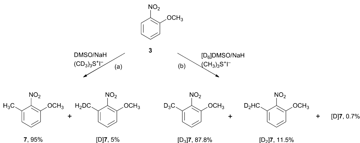
Scheme 2 Methylation of 2-nitroanisole ( 3 ) with dimethylsulfonium methylide prepared from (CD 3 ) 3 S + I − in DMSO (a) and (CH 3 ) 3 S + I − in [ D 6 ] DMSO (b).
