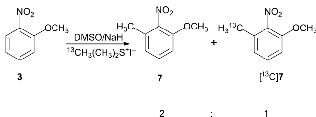
Scheme 4 Methylation of 2-nitroanisole with DMSO/NaH/ 13 CH 3 -(CH 3 ) 2 S + I - .
