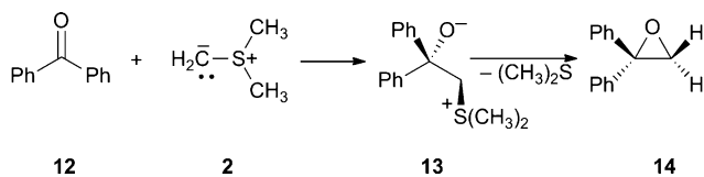
Scheme 8 Corey–Chaykowsky reaction.
