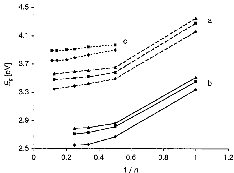
Fig. 5. Correlations of the HOMO-LUMO gaps in iso-PTAs 5 and 3a-d (series a), iso-PTAs 1a-d (series b) [2], and iso-PDAs 2b-i (series c) [3d]. \blacktriangle Corresponds to \lambda_{\max} , \blacksquare to \lambda at \epsilon_{\max}/2 , and \blacklozenge to \lambda_{\text{ig}} .
