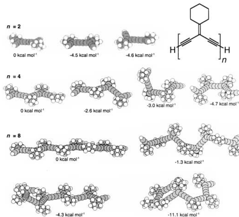
Fig. 7. PM3-Optimized structures of iso-PTA oligomers 3a , c , d . The (i-Pr) 3 Si terminal groups are replaced in the calculations by H-atoms. Energies are given relative to the near-planar all- s-trans conformation of the oligomer.
