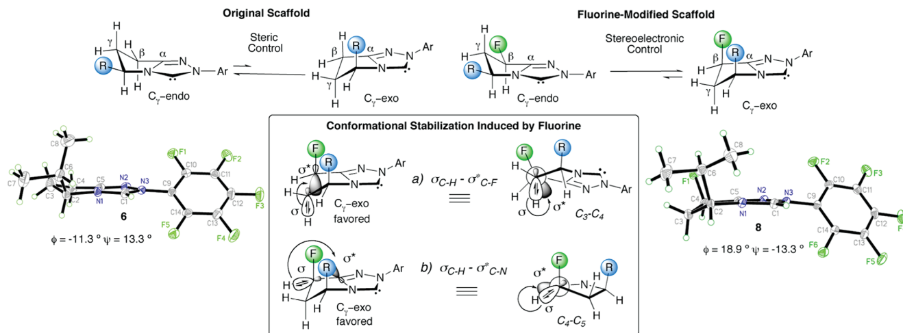
Figure 1. Conformational analysis of fluorine-modified and nonmodified triazolium salts. Conformations determined by X-ray analysis; BF 4 counterion omitted for clarity. \phi and \psi = torsion angles ( \phi = C 5 –N 1 –C 2 –C 3 ; \psi = N 1 –C 5 –C 4 –C 3 ).
