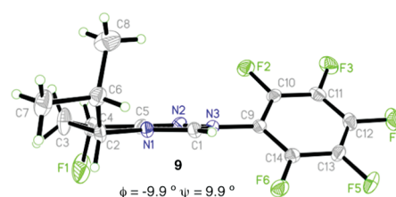
Figure 2. X-ray analysis of 9 . Conformations determined by X-ray analysis; BF 4 counterion omitted for clarity. \phi and \psi = torsion angles ( \phi = C 5 –N 1 –C 2 –C 3 ; \psi = N 1 –C 5 –C 4 –C 3 ).
