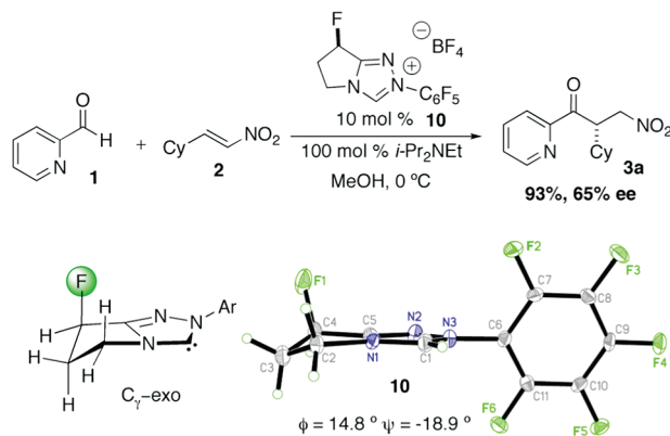
Figure 4. Examination of fluorinated triazolium salt 10 . Conformations determined by X-ray analysis; BF 4 counterion omitted for clarity. \phi and \psi = torsion angles ( \phi = C 5 –N 1 –C 2 –C 3 ; \psi = N 1 –C 5 –C 4 –C 3 ).
