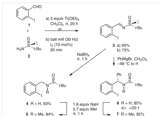
Scheme 1 Synthesis of sulfinamide-based chiral iodoarenes
