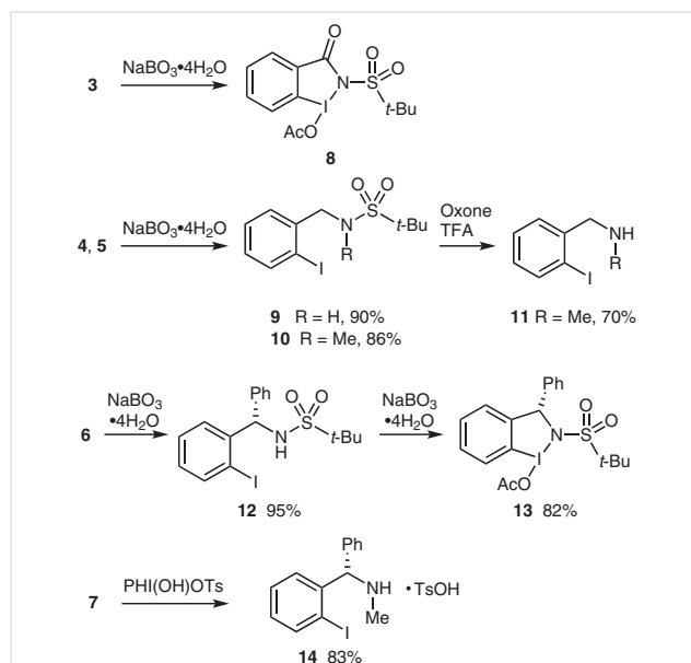
Scheme 2 Oxidation of sulfinamide-based iodoarenes 3–7
