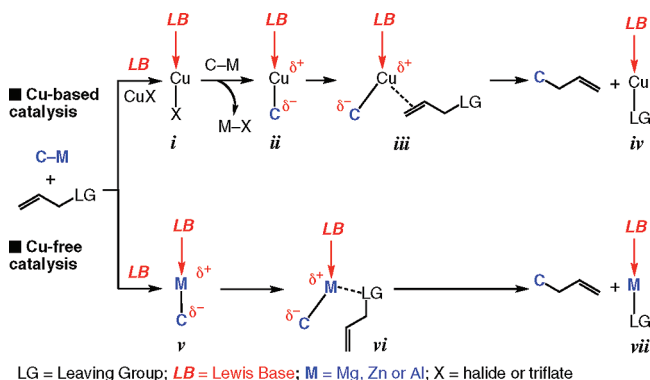
Scheme 1. Lewis Base Activation in Cu-Based and Cu-Free Pathways to Catalytic Allylic Alkylation
