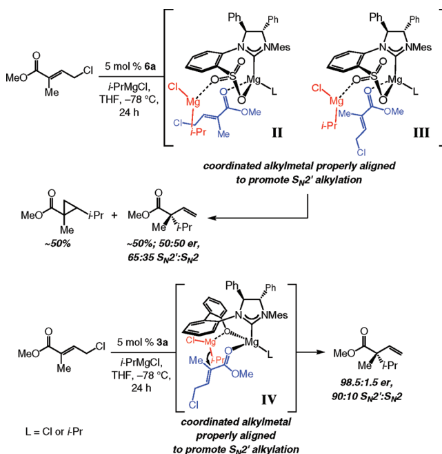
Scheme 5. Effect of Structure on the Ability of Bidentate NHC Complexes to Serve as Catalysts
