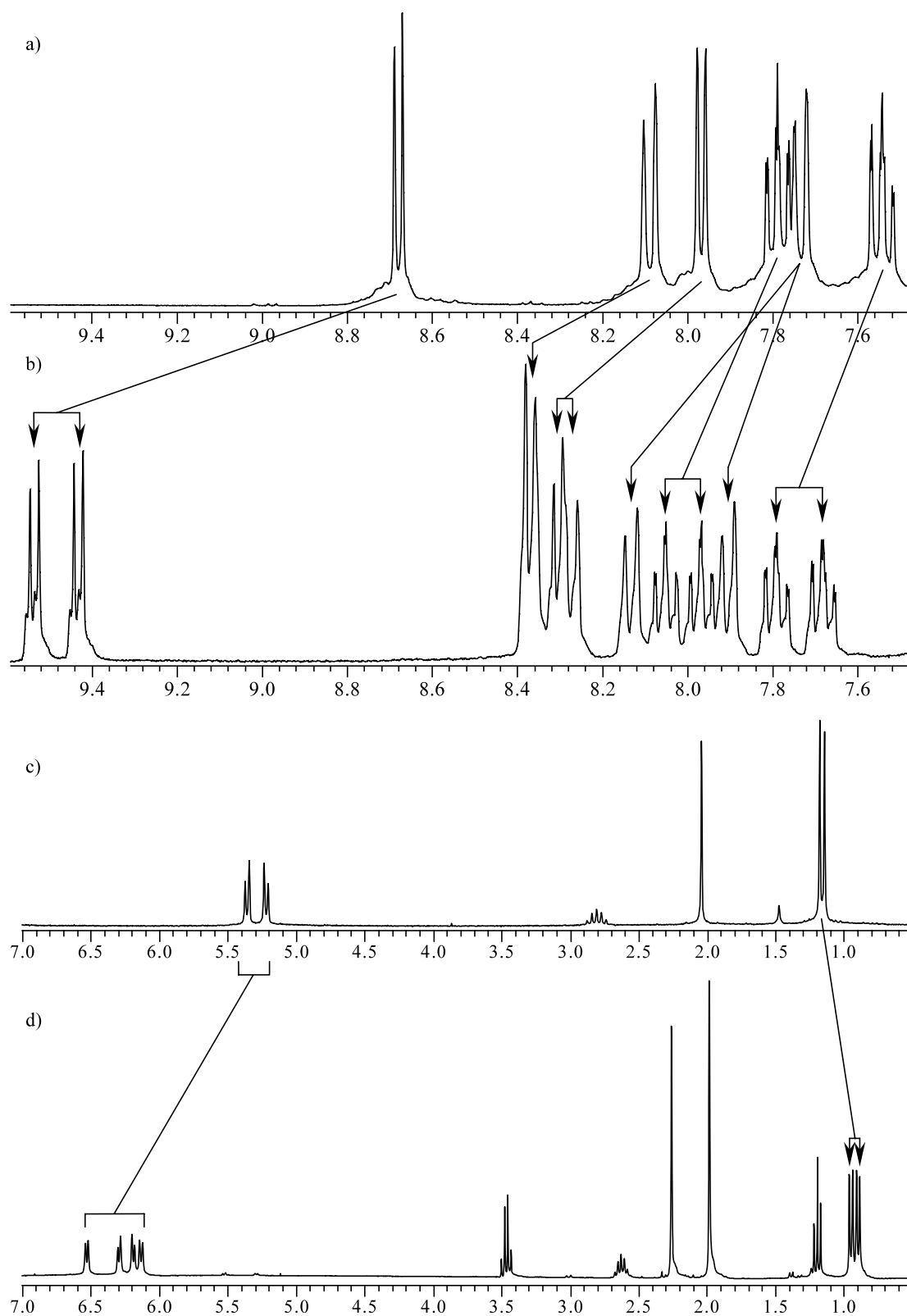
Fig. 2. ^1\text{H} -NMR of (a) biisoq (acetone- d_6 , 9.6–7.5 ppm), (b) [\text{Ru}(\eta^6\text{-}p\text{-cymene})(\text{Cl})(\text{biisoq})][\text{B}(\text{C}_6\text{H}_5)_4] ( 4b ) (acetone- d_6 , 9.6–7.5 ppm), (c) [\text{Ru}(\eta^6\text{-}p\text{-cymene})(\text{Cl})_2]_2 ( \text{CDCl}_3 , 7.0–0.5 ppm), (d) [\text{Ru}(\eta^6\text{-}p\text{-cymene})(\text{Cl})(\text{biisoq})](\text{Cl}) \cdot 0.5\text{Et}_2\text{O} ( 4a ) ( \text{CDCl}_3 , 7.0–0.5 ppm).
