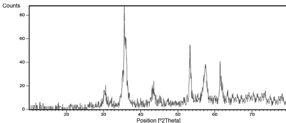
Fig. 1. The XRD pattern of \text{Fe}_3\text{O}_4 nanoparticles.
