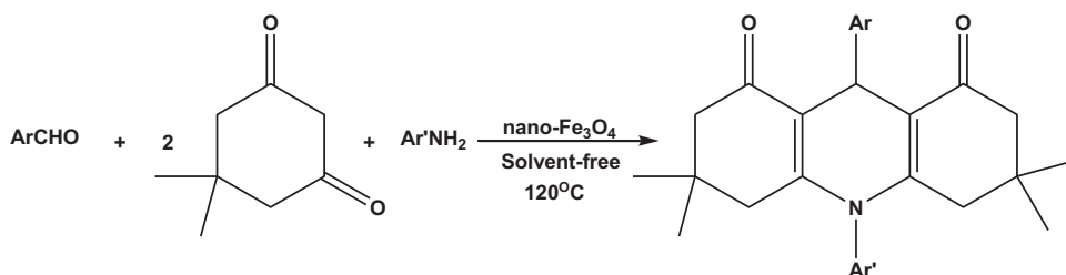
Scheme 1. Three-component reaction of aldehydes, dimedone and amines catalyzed by \text{Fe}_3\text{O}_4 nanoparticles.
