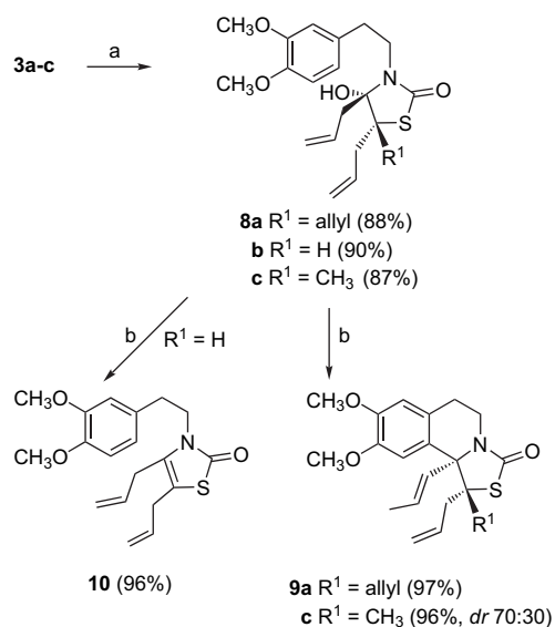
Scheme 3. Reagents: (a) allylMgCl, THF, -78^{\circ}\text{C} , 6 h. (b) TFA, CH 2 Cl 2 , reflux, 3–4 days.
