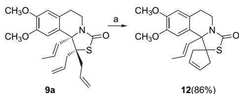
Scheme 5. Reagents: (a) second generation Grubbs' catalyst 11 , \text{CH}_2\text{Cl}_2 , reflux.
