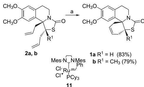
Scheme 4. Reagents: (a) second generation Grubbs' catalyst 11 (10 mol %), \text{CH}_2\text{Cl}_2 , reflux, 12 h.
