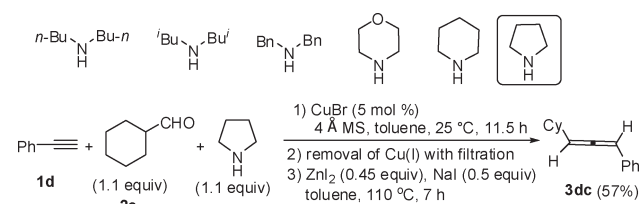
Scheme 2. Amines Screened and Preparation of Racemic 3dc
