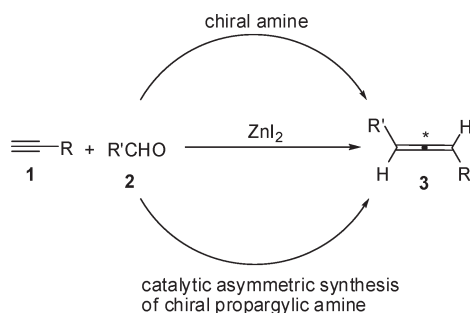
Scheme 1. Concepts for the Synthesis of Optically Active Allenes
