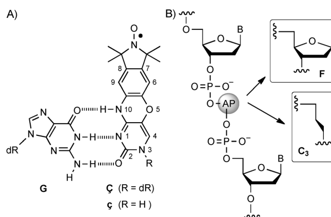
Scheme 1. A) Base pairing between guanine G and the spin-labeled nucleoside \zeta (or nucleobase c ). B) Structures of the abasic sites used in this study. AP = apurinic or apyrimidinic site. B = nucleobase.
