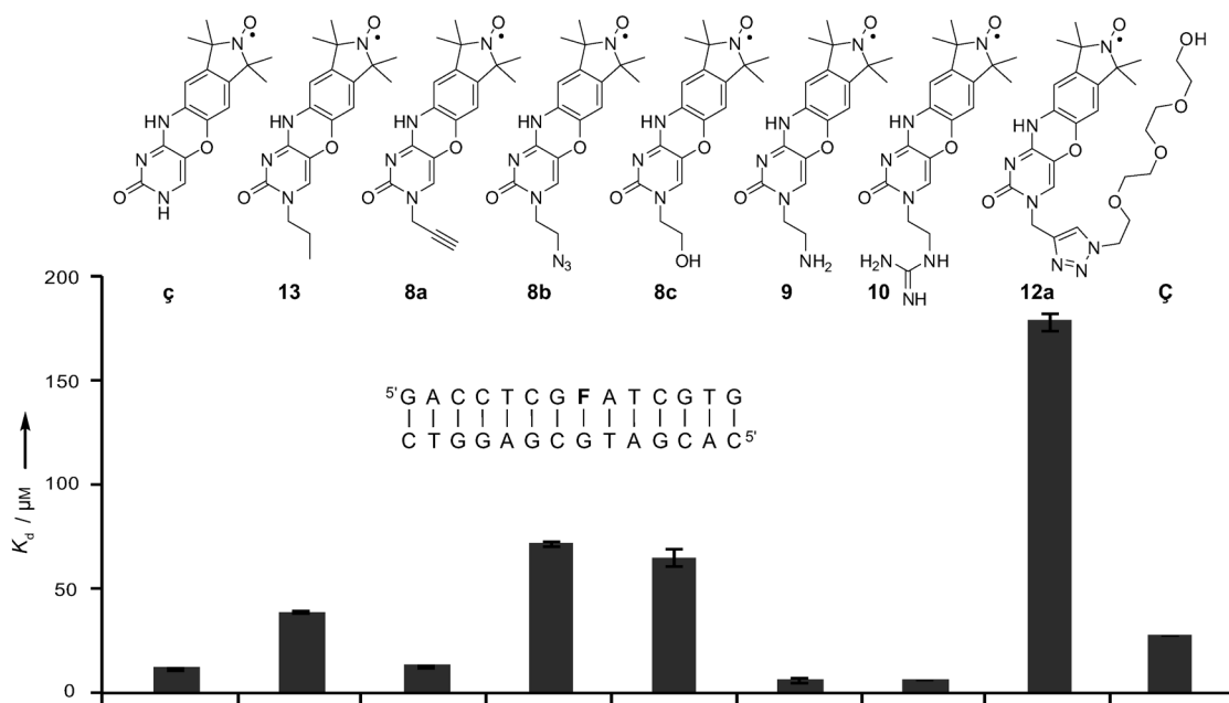
Figure 1. Structures of N3 derivatives of the spin label ζ (top). Dissociation constants (bottom) upon binding to a DNA duplex containing the abasic site F as determined from EPR data collected at –10 °C. The structure of ζ is shown in Scheme 1.
