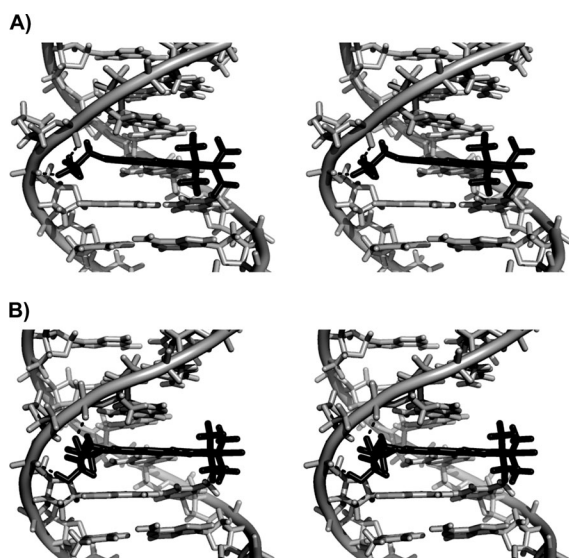
Figure 2. Stereo views of molecular models of A) spin label 9 and B) spin-labeled nucleoside \zeta (black) bound noncovalently to duplex DNA (gray) that contains an abasic site. Hydrogen bonds between the ammonium group of 9 or the hydroxyls on the 2'-deoxyribose of \zeta with non-bridging oxygen atoms of the phosphate backbone are shown as dotted lines. During the energy minimization, the sugar-phosphate backbone around the abasic site and the spin label side chains were allowed to move, while the rest of the structure was constrained.
