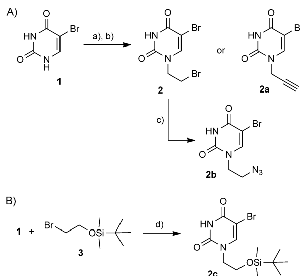
Scheme 2. Regioselective N1 modification of 5-bromouracil. a) HMDS, TMS-Cl; b) BrCH 2 CH 2 Br or BrCH 2 C≡CH, I 2 , 40–75%; c) NaN 3 , 80%; d) K 2 CO 3 , 30%.
