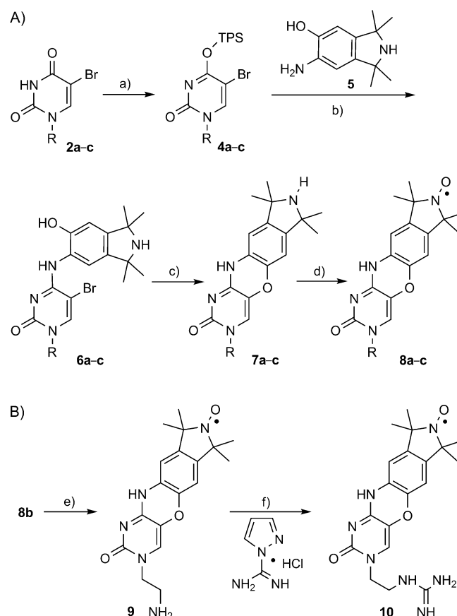
Scheme 3. Syntheses of N3 derivatives of \zeta containing polar functional group side-chains. a: R = CH 2 C≡CH; b: R = CH 2 CH 2 N 3 ; 2c , 4c , 6c : R = CH 2 CH 2 O-TBDMS; 7c , 8c : R = CH 2 CH 2 OH. a) TPS-Cl, DMAP, Et 3 N, 30–70%; b) Et 3 N, 50–70%; c) CsF, 50%; d) mCPBA, 50–65%; e) PPh 3 , 80%; f) DIPEA, 50%.
