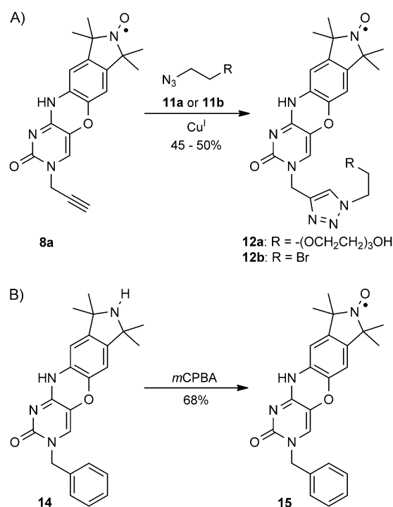
Scheme 4. A) Modification of spin label 8a by a Cu I -catalyzed Huisgen–Meldal–Sharpless [3+2] cycloaddition. B) Synthesis of an N3-benzyl derivative of spin label ζ .
