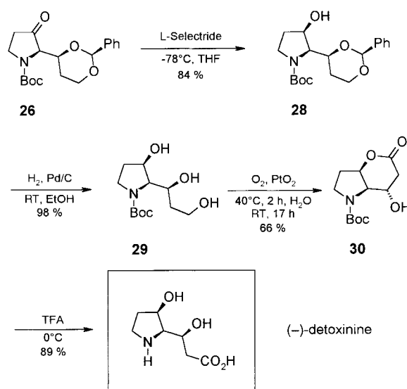
Scheme 9. Completion of the total synthesis of (–)-detoxinine.
