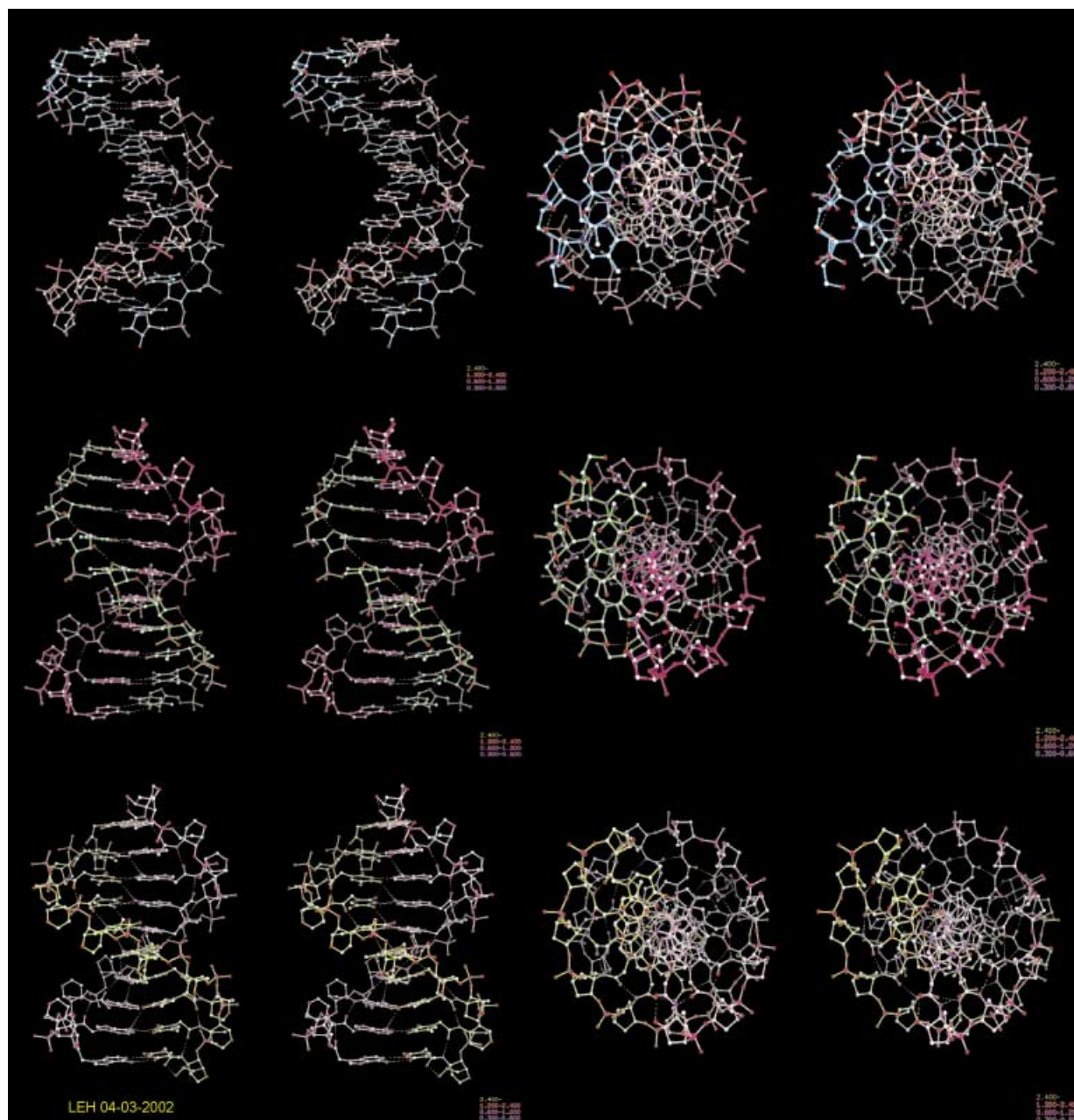
Figure 9. Stereoview of duplexes perpendicular and parallel to the helix axis. Top: right-handed \text{bca}(\text{A}_{10}) \cdot \text{r}^{\text{D}}(\text{T}_{10}) ; middle: left-handed \text{bca}(\text{A}_{10}) \cdot \text{r}^{\text{L}}(\text{T}_{10}) ; bottom: left-handed \text{bca}(\text{A}_{10}) \cdot \text{bca}(\text{T}_{10}) .
