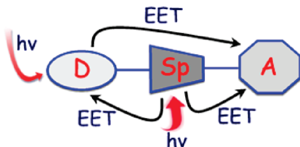
Scheme 1. Pictorial Illustration of EET in the Linear Triads Described Herein, Where D, Sp and A, Respectively, Refer to Donor, Spacer and Acceptor
