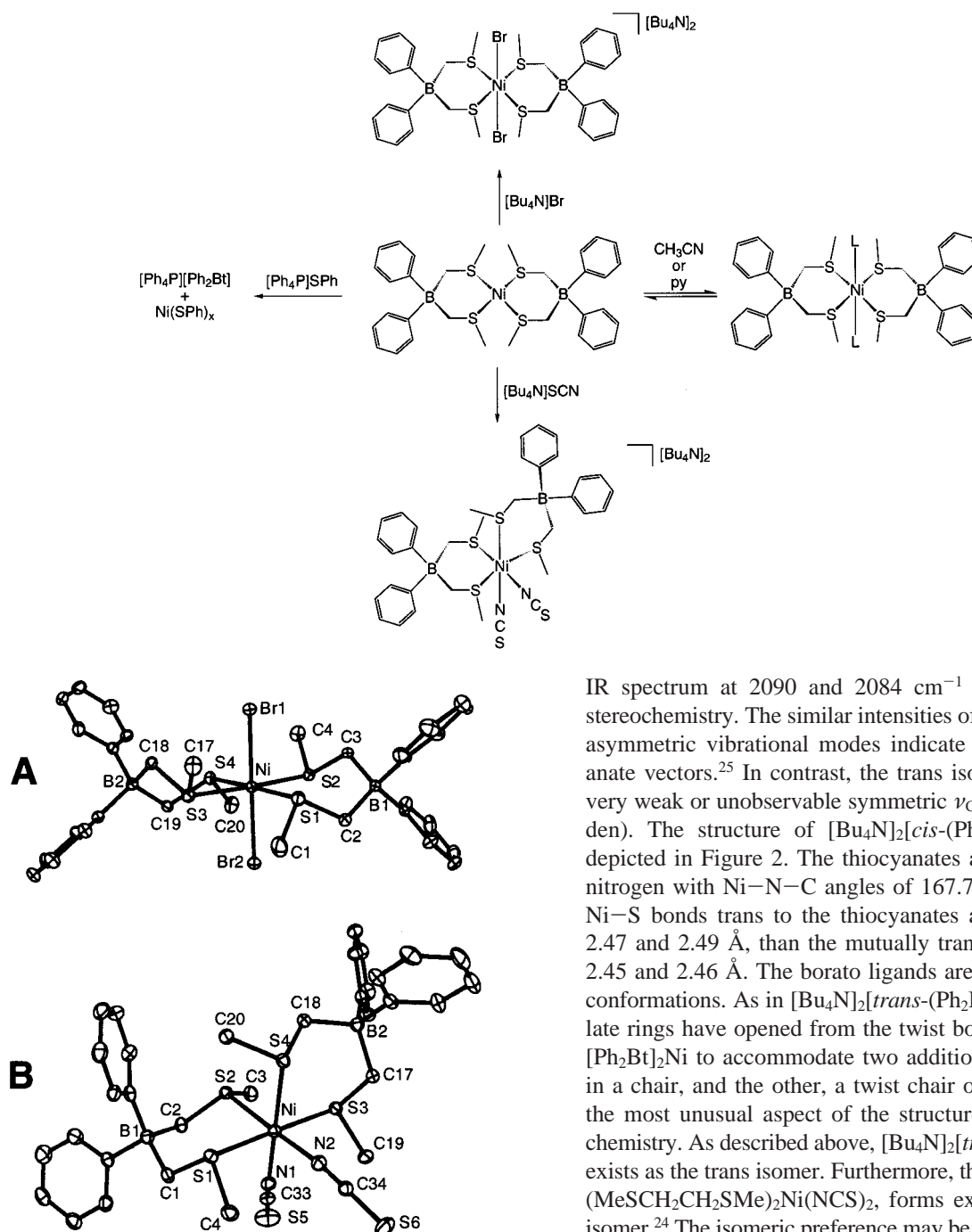
Figure 2. Thermal ellipsoid plots of anions of [\text{Bu}_4\text{N}]_2[\text{trans}-(\text{Ph}_2\text{Bt})_2\text{NiBr}_2] (A) and [\text{Bu}_4\text{N}]_2[\text{cis}-(\text{Ph}_2\text{Bt})_2\text{Ni}(\text{NCS})_2] (B) at 30% probability level; hydrogen atoms not shown.
