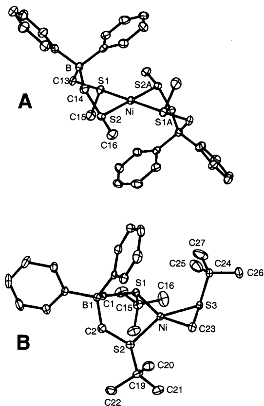
Figure 1. Thermal ellipsoid plots of [Ph 2 Bt] 2 Ni (A) and [Ph 2 Bt tBu ] 2 Ni( \eta^2 -CH 2 SBu t ) (B) at 30% probability level; hydrogen atoms not shown.
