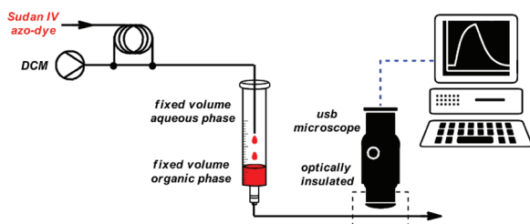
Fig. 3 Flow setup for dispersion measurements.
