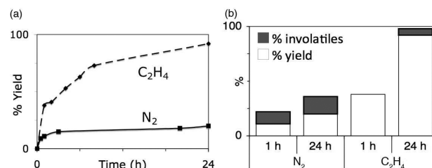
Figure 1. (a) Rates of RCEYM for the reaction of Scheme 1; (b) product distribution under \text{C}_2\text{H}_4 , vs \text{N}_2 atmosphere; in situ yields determined by calibrated GC–FID analysis.
