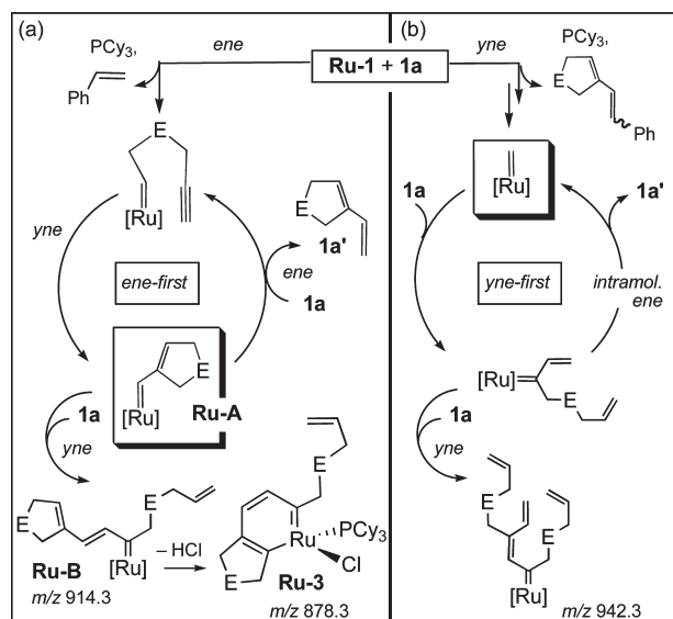
Scheme 2. (a) Ene-First versus (b) Yne-First RCEYM, Showing Productive Cyclization, Uptake of a Second Enyne, and (for the Ene-First Pathway), Formation of Deactivated Ru-3 a
