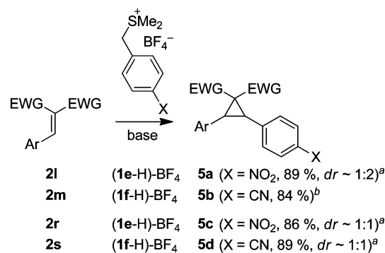
Scheme 5. Reactions of the Semistabilized Sulfur Ylides 1e–g and the Stabilized Sulfur Ylide 1h with Different Michael Acceptors
