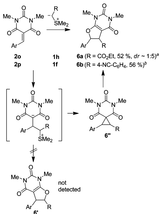
Scheme 6. Reactions of the Sulfur Ylides 1f and 1h with the Benzylidenemalbarbituric Acids 2o and 2p
