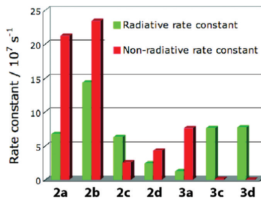
Figure 7. Rate constants of the tetracene series 2 and 3 in \text{CH}_2\text{Cl}_2 .
