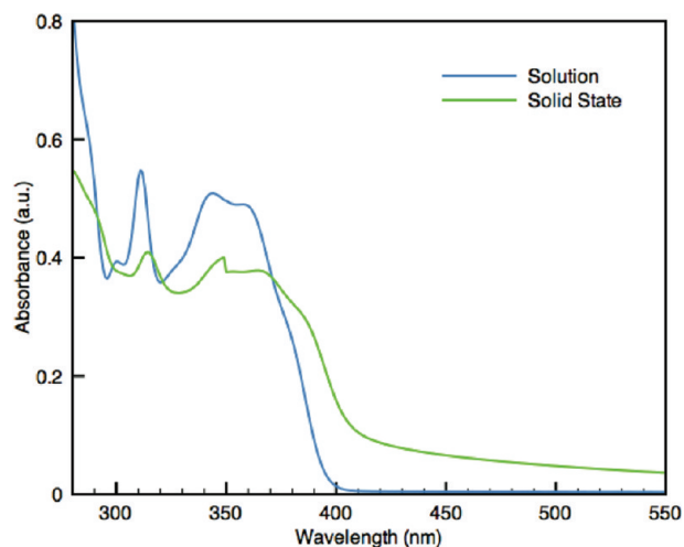
Figure 14. Absorption of the fibers of 4a , as solid and dissolved in \text{CH}_2\text{Cl}_2 .
