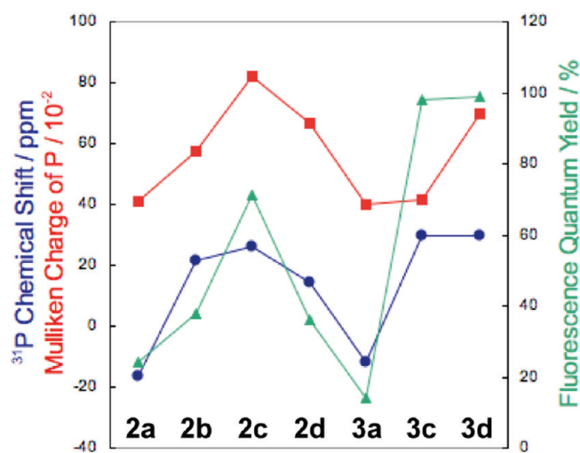
Figure 9. Trends between fluorescence quantum yield and the electronic nature of phosphorus; red: DFT calculated Mulliken charge of P/10 −2 ; blue: 31 P NMR shift (CDCl 3 at 298 K)/ppm; green: fluorescence quantum yield/%.
