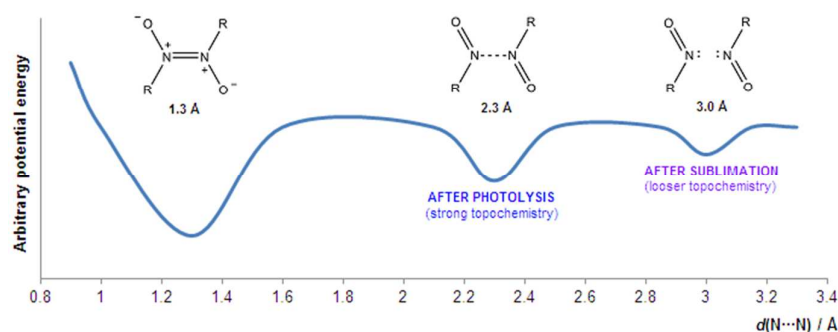
Fig. 2 The nitrogen-nitrogen atom distances in three different potential energy minima corresponding to covalent bond (azodioxide), closed packed monomers in photolysed sample,
