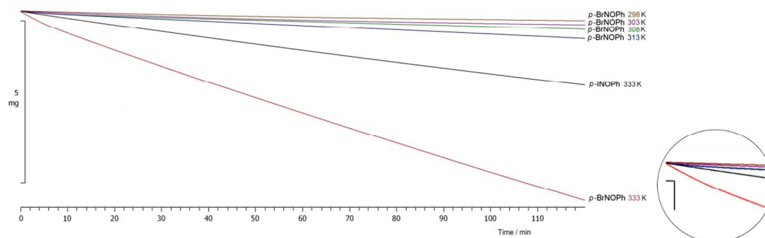
Fig. 3 Isothermal TGA diagrams for p -bromo- and p -iodinitrosobenzene crystals. The loss of mass is caused by removing the material by sublimation. The first ten minutes are extrapolated in the circle on the right. The y-axis shows the relative weight scale (only in 5 mg range).
