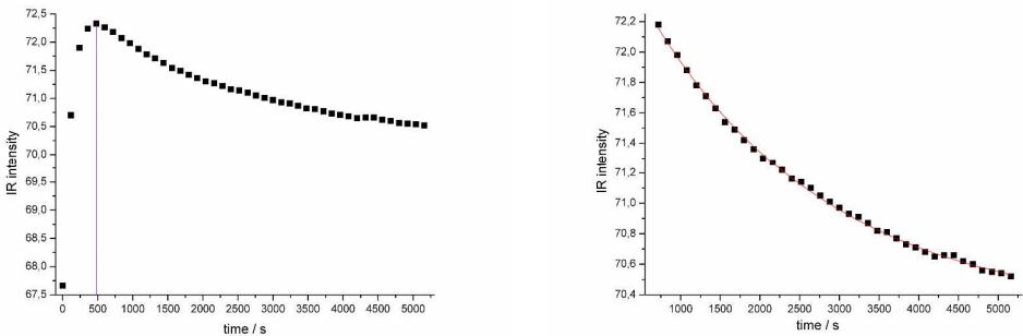
Fig. 4 Change in intensities of the monomer ( \nu(\text{NO})=1489\text{ cm}^{-1} ) during solid-state dimerization of the p -bromonitrosobenzene at 25 °C measured by time-resolved FTIR. Intensity change during incubation period (left) and reaction period (right)
