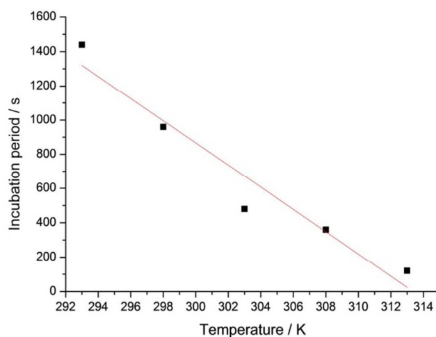
Fig. 5 Dependence of the incubation period for the solid-state dimerization on the temperature.
