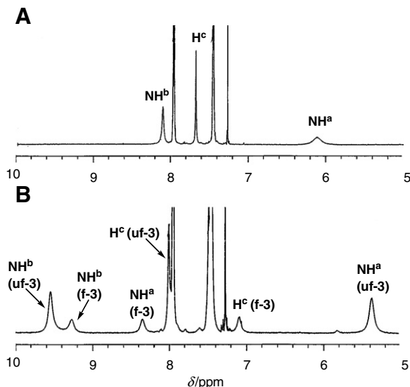
Fig. 2. ^1\text{H} NMR spectra of 3 in \text{CDCl}_3 (A) at 25^\circ\text{C} and (B) at -50^\circ\text{C} .
