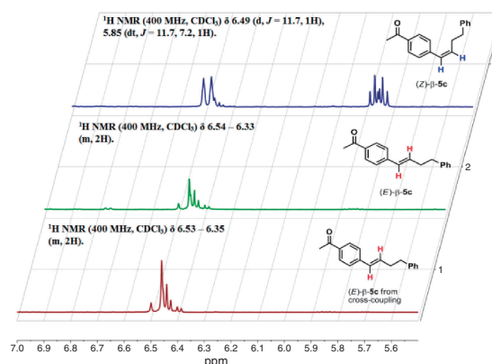
Figure 1. Comparison of 1 H NMR spectra of alkene region of: a) authentic ( Z )-β- 5c , b) authentic ( E )-β- 5c , and c) ( E )-β- 5c from cross-coupling of alkenylgermane 3a with 4-AcC 6 H 4 Br (Entry 3, Table 1).
