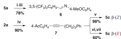
Scheme 3. Experiments to confirm the regio- and stereochemical assignments of styrenyl cross-coupling products 5a and 5c . Conditions: i) O 3 , CH 2 Cl 2 , –78 °C, 10 min; ii) PPh 3 (2.5 equiv), CH 2 Cl 2 , 0–23 °C, 1 h; iii) 4-anisidine (1.5 equiv), CH 2 Cl 2 , 2 h; iv) 4-AcC 6 H 4 I (1.0 equiv), [PdCl 2 (PPh 3 ) 2 ] (3 mol %), TBAF (2 equiv), CuI (3 mol %), THF, 16 h; v) H 2 (1 atm), Lindlar's catalyst (Pd/Pb), EtOAc, 2 h; vi) [Cp* + Ru(MeCN) 3 ] + PF 6 – (1 mol %), (EtO) 3 SiH (1.2 equiv), CH 2 Cl 2 , 16 h; vii) CuI (1.5 equiv), TBAF (3 equiv), THF, 16 h.
