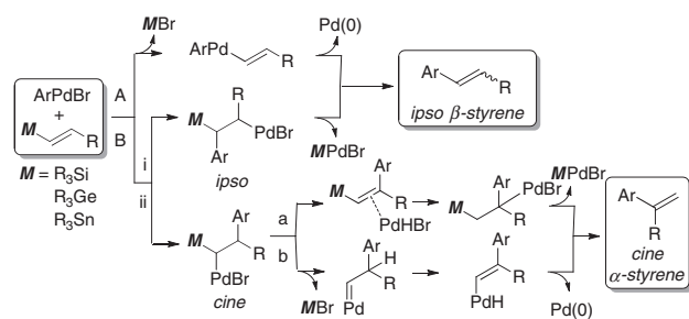
Scheme 4. Proposed reaction pathways for alkenyl group 14 metal cross-coupling reactions.
