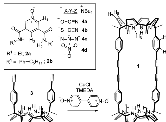
Scheme 1. Synthetic Scheme for the Preparation of Macrocycle 1 and Structures of Bis-amidepyridyl- N -oxides 2 and the Tetrabutylammonium Ion-Pairs of Polyatomic Anions 4
