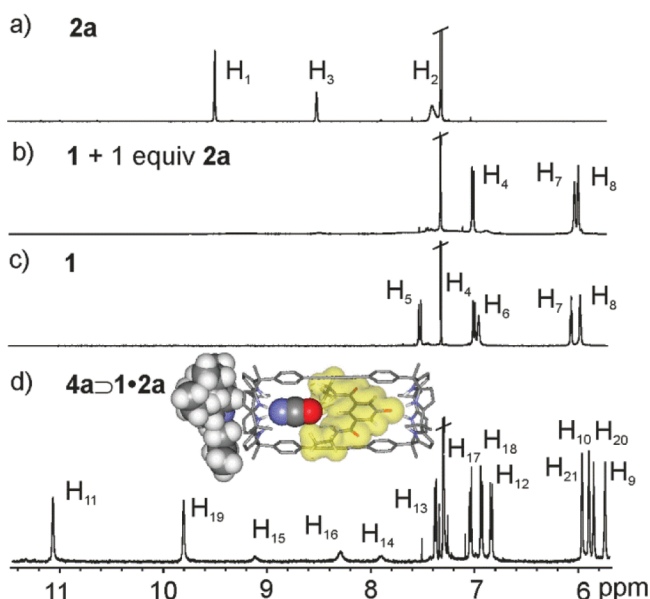
Figure 1. Downfield regions of the ^1\text{H} NMR spectra (500 MHz, \text{CDCl}_3 , 298 K) of the free linear 2a (a) and cyclic 1 (c) components of the pseudorotaxanes, its equimolar mixture (b) and the solution containing the three components 1 , 2a , and 4a in a 1:1:1 ratio (d). Inset: CAChe minimized structure of ion-paired [2]pseudorotaxane complex 4a ⊃ 1 · 2a . See Schemes 1 and 2 for proton assignments.
