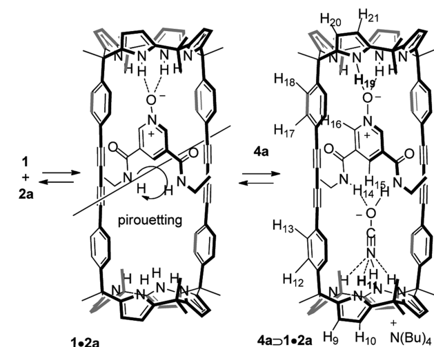
Scheme 2. Two-Step Quantitative Self-Assembly of 4a ⊃ 1 · 2a
