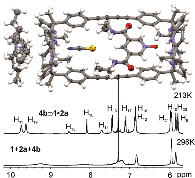
Figure 2. (Top) Single-crystal X-ray structure of 4b \supset 1 \cdot 2a . 27 (Bottom) Downfield regions of the 1 H NMR spectra of the CDCl 3 solution containing an equimolar mixture of 1 , 2a , and tetrabutylammonium thiocyanate 4b recorded at 298 and 213 K. [ 1 ] = [ 2a ] = [ 4b ] = 4.6 \times 10^{-3} \text{ M} .
