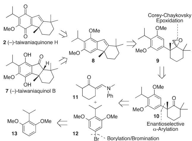
Scheme 1. Retrosynthetic Analysis for the Syntheses of (–)-Taiwaniaquinone H (2) and (–)-Taiwaniaquinol B (7)
