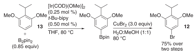
Scheme 2. One-Pot Synthesis of Aryl Bromide 12 a
