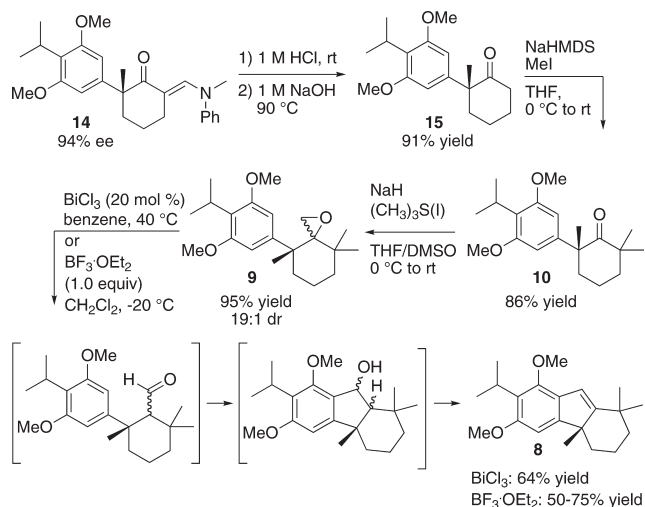
Scheme 3. Synthesis of Tetrahydrofluorene 8
