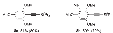
Figure 2. Alkynylation of trimethoxybenzenes. Reaction conditions: 0.40 mmol trimethoxybenzene, 0.56 mmol 1 , 0.02 mmol AuCl in 2 mL i PrOH at 60 °C under air. Isolated yields. Yields based on recovered starting materials under parentheses.
