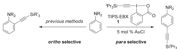
Scheme 1. Direct Alkynylation of Anilines
