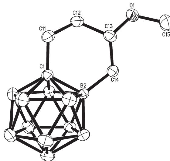
Figure 1. Molecular structure of the anion [1,2-(CH 2 ) 2 CH(OMe)CH 2 -1-CB 11 H 10 ] − in [Me 3 NH][ 2b ] (all H atoms are omitted for clarity). Selected bond lengths [Å]: C1–C11 1.528(3), C11–C12 1.520(3), C12–C13 1.510(4), C13–C14 1.517(3), C14–B2 1.594(3), B2–C1 1.718(3), and C13–O1 1.455(3).
