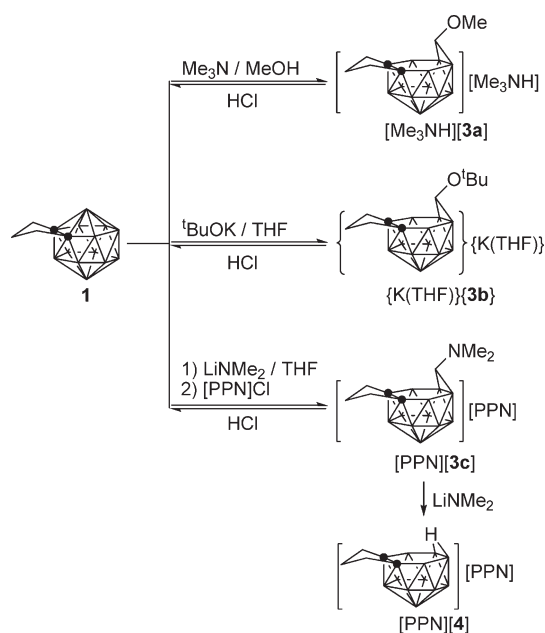
Scheme 3. Reaction of 1 with Nucleophiles
