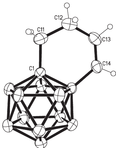
Figure 2. Molecular structure of the anion [1,2-(\text{CH}_2)_2\text{CH}=\text{CH}-1-\text{CB}_{11}\text{H}_{10}]^- in [\text{Me}_3\text{NH}][2\text{c}] (the H atoms of all BH vertices are omitted for clarity). Selected bond lengths [Å]: C1–C11 1.537(6), C11–C12 1.445(8), C12–C13 1.498(9), C13–C14 1.319(7), C14–B2 1.572(6), and B2–C1 1.690(6).
