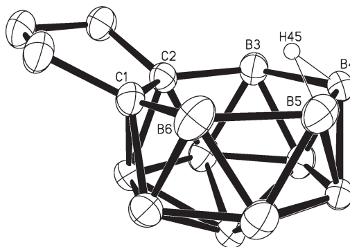
Figure 5. Molecular structure of the anion [8,9-(\text{CH}_2)_3-8,9-\text{C}_2\text{B}_{11}\text{H}_{12}]^- in [\text{PPN}][4] (all H atoms are omitted for clarity). Selected bond lengths [Å]: C1–C2 1.557(3), C2–B3 1.603(4), B3–B4 1.788(4), B4–B5 1.817(5), B5–B6 1.795(5), and B6–C1 1.607(4).
