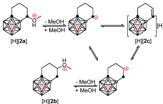
Scheme 2. Possible Mechanism for the Interchange among [2\text{a}]^- , [2\text{b}]^- , and [2\text{c}]^-
