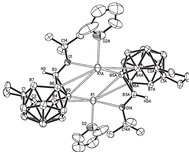
Figure 3. Molecular structure of \{\text{K}(\text{THF})\}\{8,9-(\text{CH}_2)_3-\mu-11,12-(t\text{BuO})\text{BH}-8,9-\text{C}_2\text{B}_{11}\text{H}_{11}\} ( \{\text{K}(\text{THF})\}\{3\text{b}\} ) (all H atoms are omitted for clarity). Selected bond lengths [Å]: B3–O1 1.390(5), B3–B5 1.879(5), B3–B6 1.879(5), C1–C2 1.529(5), C2–B4 1.647(5), B4–B5 1.774(5), B5–B6 1.779(5), B6–B7 1.770(6), and B7–C1 1.655(6).
