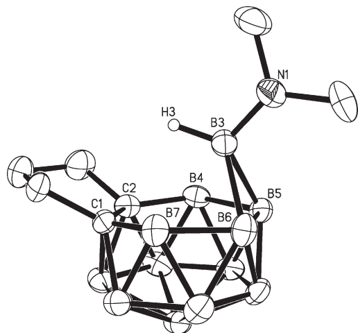
Figure 4. Molecular structure of the anion [8,9-(\text{CH}_2)_3-\mu-11,12-(\text{Me}_2\text{N})\text{BH}-8,9-\text{C}_2\text{B}_{11}\text{H}_{11}]^- in [\text{PPN}][3\text{c}] (all H atoms are omitted for clarity). Selected bond lengths [Å]: N1–B3 1.414(4), B3–B5 1.888(4), B3–B6 1.891(5), C1–C2 1.547(3), C2–B4 1.628(4), B4–B5 1.786(5), B5–B6 1.783(4), B6–B7 1.781(4), and B7–C1 1.627(4).
