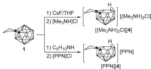
Scheme 4. Synthesis of nido 13-Vertex Carborane Anions [4]^-
