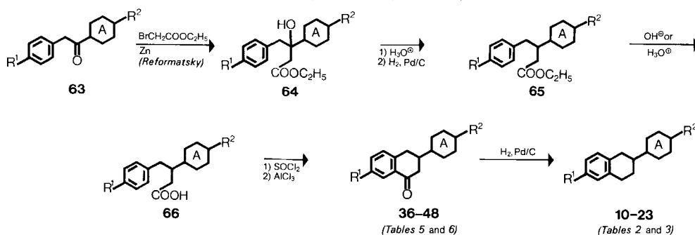
Scheme 4 (see Tables 2, 3, 5 and 6)
