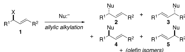
Figure 1. Issues of selectivity in modern allylic alkylation.
