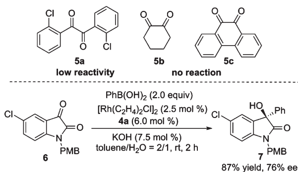
Scheme 2. Rh(I)-Catalyzed Asymmetric Addition to Other \alpha -Diketones or Isatins
