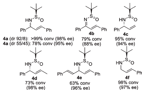
Figure 1. Evaluation of representative chiral sulfur–alkene hybrid ligands for Rh(I)-catalyzed asymmetric addition to benzil ( 1a ).
