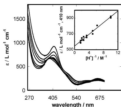
Figure 9. The change in the absorption spectrum of L410 with acid concentration. Reading downward at 410 nm, [\text{H}^+] is 0.10, 0.16, 0.20, 0.30, 0.40, 0.50, and 0.60 \text{ mol L}^{-1} . Inset: plot of \bar{\epsilon}_{410} versus [\text{H}^+]^{-1} .
