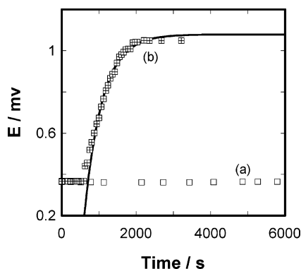
Figure 7. Experiments showing hydrogen evolution from Eu 2+ acidic solution catalyzed by MeReO 3 . Conditions: 12.8 mmol L -1 Eu 2+ , 0.22 mol L -1 H + , and \mu = 0.29\text{ mol L}^{-1} . (a) The control experiment without MeReO 3 . (b) Experiment with 0.193 mmol L -1 MeReO 3 . The time lag in hydrogen evolution is the “inertia” in moving the Hg plug at the beginning.
