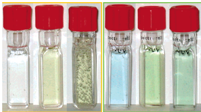
Figure 2. Visual changes in acidic solution, from left to right: 12 mmol L -1 Eu 2+ ; 12 mmol L -1 Eu 2+ with 0.3 mmol L -1 MeReO 3 after 1 min; 30 min later, showing hydrogen evolution; 12 mmol L -1 Cr 2+ ; 12 mmol L -1 Cr 2+ with 0.3 mmol L -1 MeReO 3 after 1 min; 1 h later. All solutions contain 120 mmol L -1 HCl.
