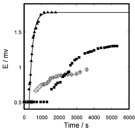
Figure 11. Plots of hydrogen evolution with both \text{Cr}^{2+}_{\text{aq}} and \text{Eu}^{2+} . Conditions: [\text{H}^+] = 0.11\text{ M} , \mu = 0.3\text{ M} , 25\text{ }^\circ\text{C} . Case 1 (○): 3.3\text{ mM Eu}^{2+} mixed with 0.19\text{ mM MTO} , and then 3\text{ mM Cr}^{2+} . Case 2 (■): 3\text{ mM Cr}^{2+} mixed with 0.19\text{ mM MTO} , and then 3.3\text{ mM Eu}^{2+} . Case 3 (▲): a comparison experiment, 3.3\text{ mM Eu}^{2+} mixed with 0.19\text{ mM MTO} , and then another 3.3\text{ mM Eu}^{2+} . Data from case 3 are fit to first-order kinetics, ignoring the time lag.
