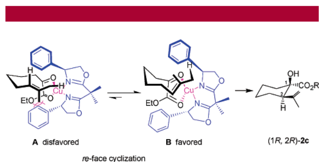
Figure 1. Proposed transition-state model for the {Cu[( S,S )-Ph-box]} complex-promoted carbonyl ene cyclization reaction of 1c .
