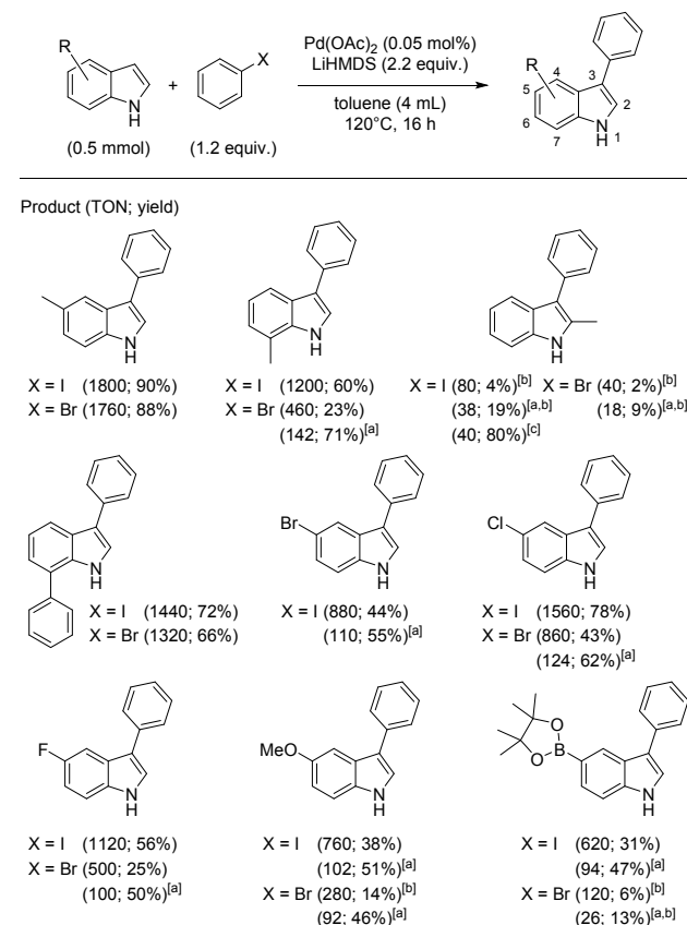
Scheme 4. Scope of functionalized indoles. TON are calculated from isolated yields if not otherwise stated. [a] 0.5 mol% of \text{Pd}(\text{OAc})_2 used. [b] TON calculated from GC-FID yield. [c] 2.0 mol% of \text{Pd}(\text{OAc})_2 used.
