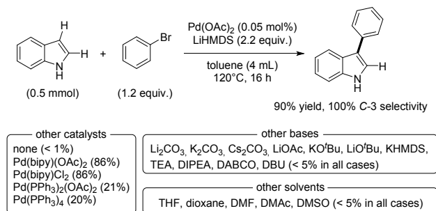
Scheme 2. The \text{Pd}(\text{OAc})_2/\text{LiHMDS} catalytic system for efficient C-3 arylation of 1 H -indole and overview of screened parameters.
