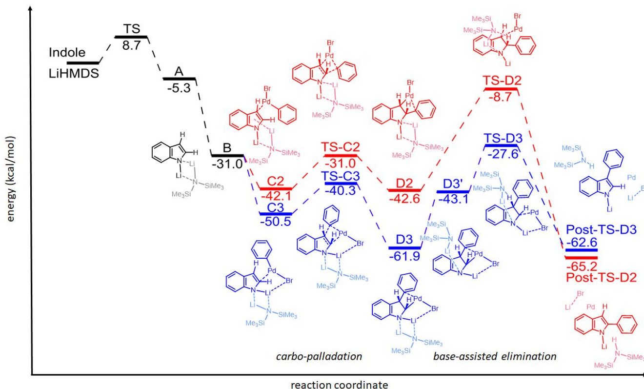
Figure 1. Schematic relative free energy profile for the reported reaction calculated at the DFT (PBE0-D3) level. Pathways towards C-2 or C-3 arylated indole are shown in red and blue, respectively. Structures of calculated intermediates and transition states are represented.
