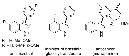
Scheme 1. API based on C-3 arylated free (NH)-indoles and their biological activity. 35–38
