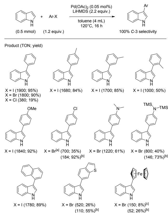
Scheme 3. Scope of aryl halides. TON are calculated from isolated yields if not otherwise stated. [a] 3 equivalents of 1-bromo-4-chlorobenzene were used. [b] 0.5 mol% of \text{Pd}(\text{OAc})_2 used. [c] TON calculated from GC-FID yield.
