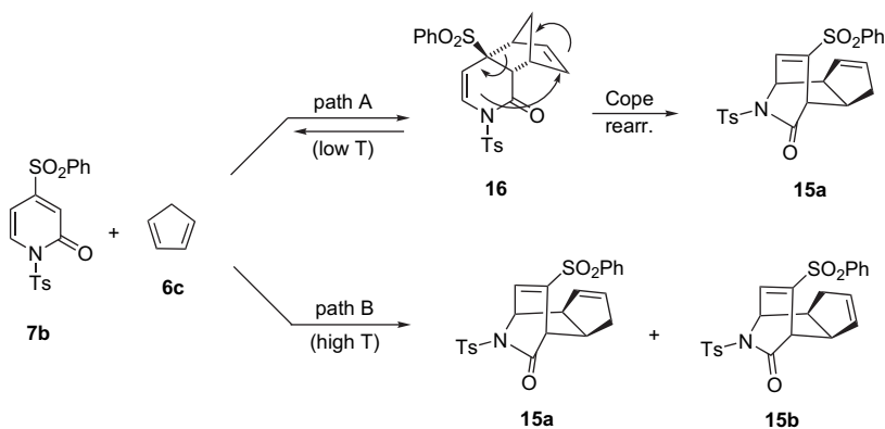
Scheme 2. Proposed pathways for the reaction of 7b with 6c .
