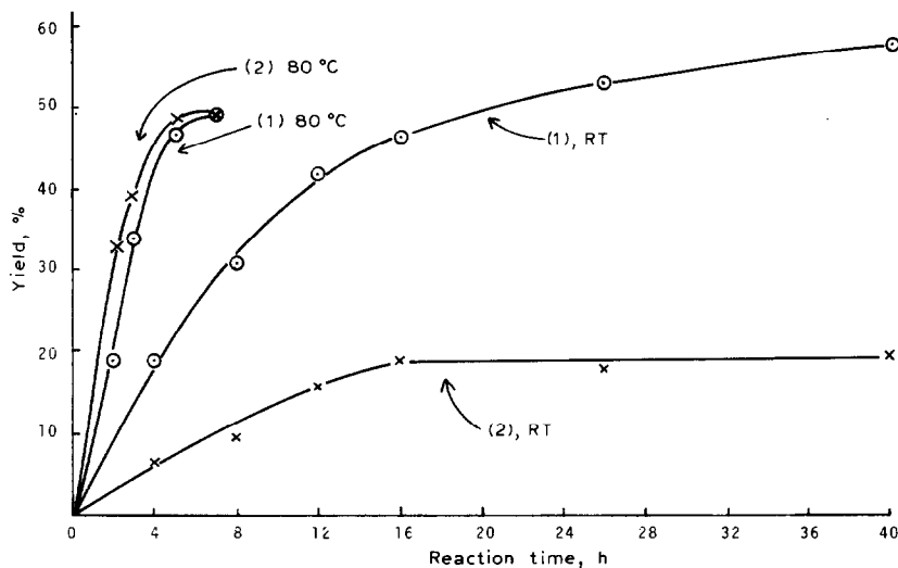
Fig. 4. Addition of triethoxysilane to acetylene catalyzed by "Si"-SH-Pt. (1) \text{CH}_2=\text{CHSi}(\text{OC}_2\text{H}_5)_3 , (2) ((\text{C}_2\text{H}_5\text{O})_3\text{SiCH}_2)_2 . S/Pt, 6; Pt, 0.026 mg atom; triethoxysilane, 34.7 mmol.
