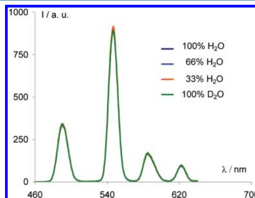
Figure 2. Tb-centered luminescence of 30 \mu\text{M} \text{TbP}^{\text{HD}2} in \text{D}_2\text{O}/\text{H}_2\text{O} mixtures HEPES buffer (10 mM, pH = 7.0).
