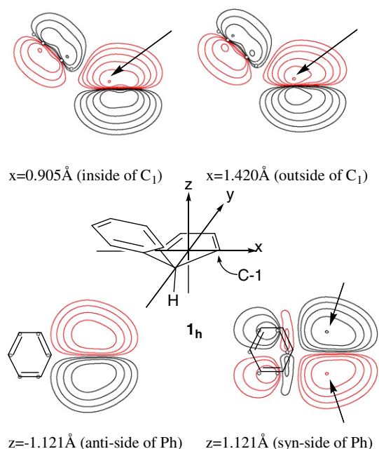
Fig. 3. Contour maps of the sections ( x = 0.905, 1.420 , and z = \pm 1.121 Å) of the FMO of the fixed conformer 1 h at the RHF/6-31G* level ( C_s ). The C_p ring is in xy plane. C_1 and C_4 carbons are on the x -axis at the space coordinates (Å) of (1.173, 0, 0) and (−1.173, 0, 0), respectively. The absolute value of the largest contour line is 5.0 \times 10^{-3} AU. The heights of adjacent contours differ by a factor 2.0.
